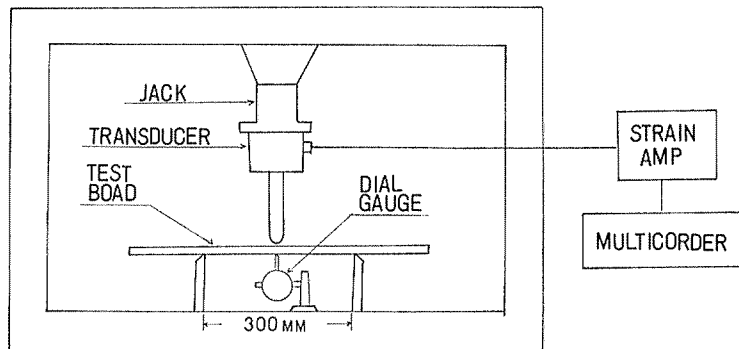
Fig. 1. Outline of the bending test system.
