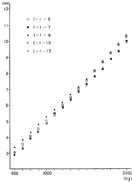
Fig. 2. Relation between bend and load. Test board No. I-1.
