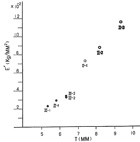
Fig. 5. Relation between stiffness ( E' ) and thickness.
