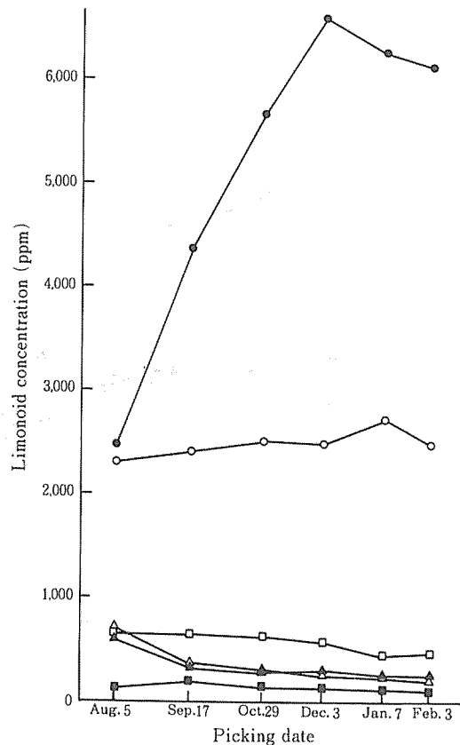
Fig. 4. Total limonoid concentrations in the component parts of Otachibana fruit.
