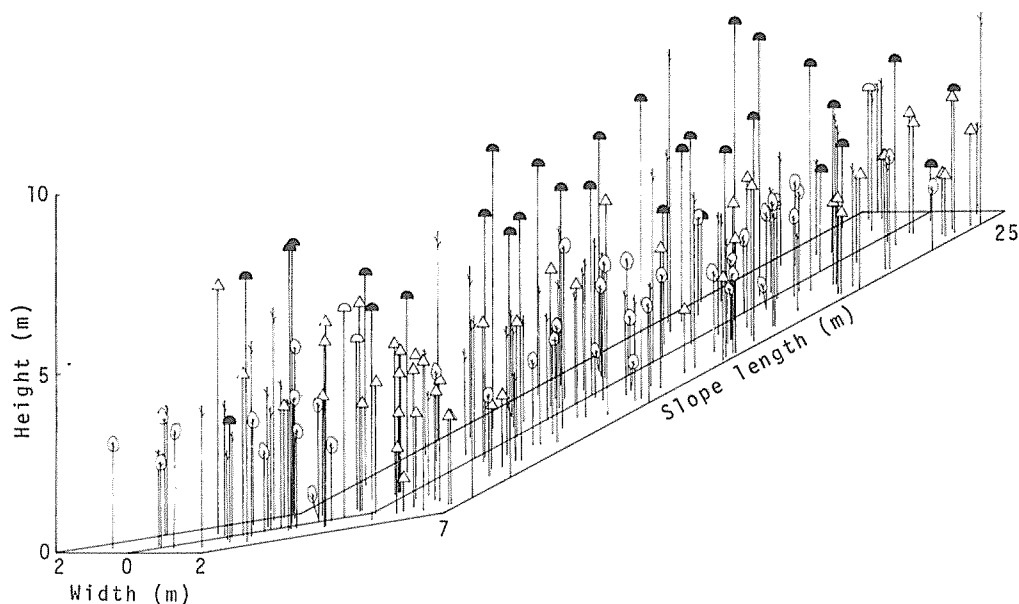
Fig. 2 Stratification of research stand and distributional structure of each tree by belt transect method in Plot 2
