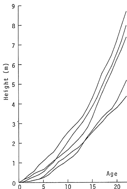
Fig. 6 Process of height growth by stem analysis of Hinoki sample trees
