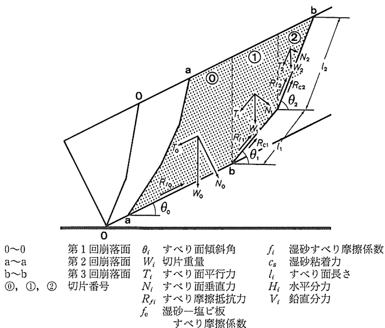
Fig. 3 Sliding friction coefficient and cohesion of wet sand.
