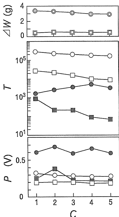
Fig. 7 Relations between repeated cycle (C) of wetting and drying and weight change ( \Delta W ), AE total event (T), and mean AE amplitude (P) for specimens of sapwood and heartwood of sugi. Each plot is the mean of three specimens.
