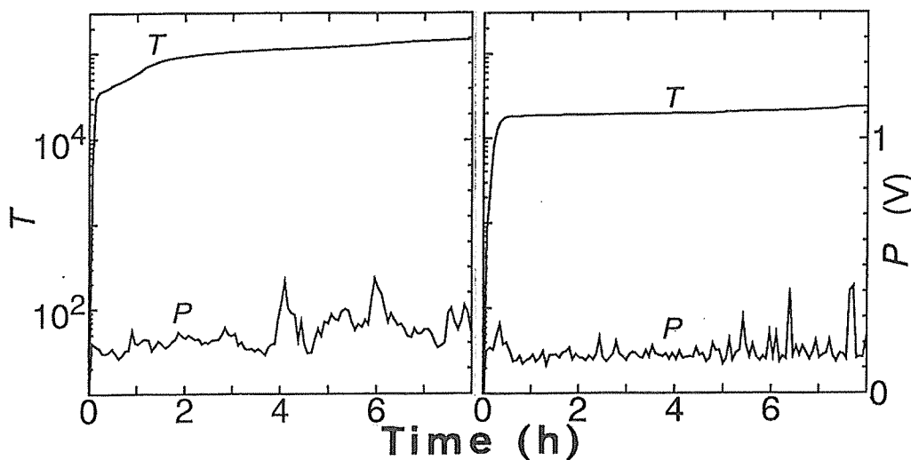
Fig.10 AE generation during wetting (left) and drying (right) of charcoal specimen. T, AE total event count; P, mean AE amplitude per 250 seconds.
