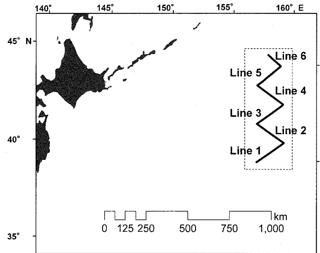
Figure 1. Study area and survey transects. Dotted rectangle indicates the study area. Black thick line shows whole survey transects. Each transect was labeled from south to north (Lines 1 to 6).
