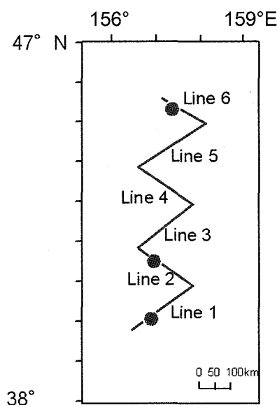
Figure 2. The survey transects and sampling stations. Black line indicates the whole transects with labels of transects. Black circles are stations with MOCNESS trawls.
