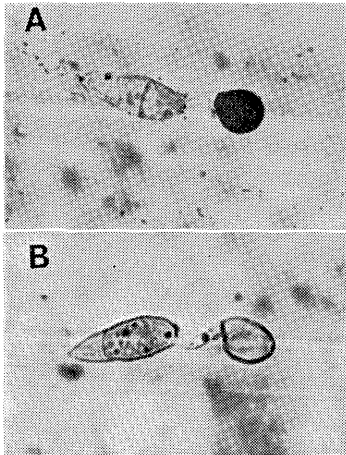
Fig. 5. Effect of IPT as observed in the morphology of appressoria. A: Normal appressorium; B: Abnormal appressorium produced in 50 ppm IPT.
