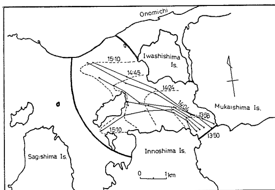
Fig. 3-2. Loci of current drogues released at the Mekari-Seto, Nov. 13, 1974, 13:50-15:10, and the tidal mixing area estimated by them (ebb tide).
