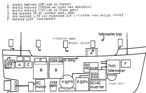
Fig. 5. Schematic diagram of arrangement of measuring apparatus for ship's motion and relative wave elevation.
