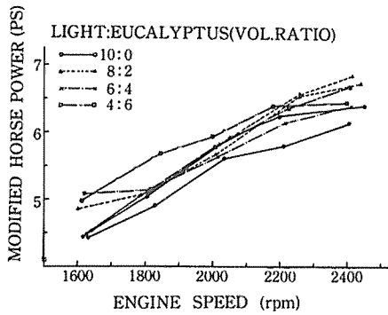
Fig. 3. — Modified horse power curve
