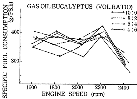
Fig. 11. — Specific fuel consumption curve
