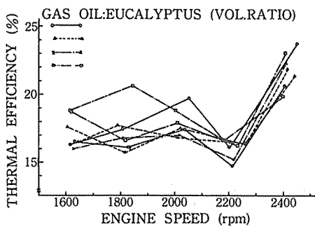
Fig. 13. — Thermal efficiency curve
