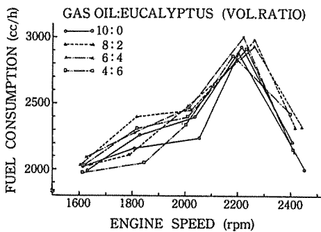
Fig. 7. — Fuel consumption curve
