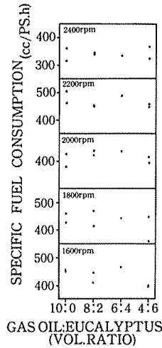
Fig. 10. — Relationships between blend ratio and specific fuel consumption
