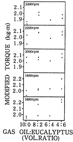
Fig. 6. — Relationships between blend ratio and modified torque
