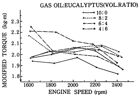
Fig. 5. — Modified torque curve
