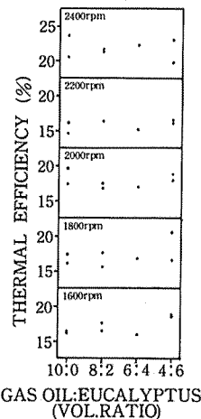
Fig. 14. — Relationships between blend ratio and thermal efficiency
