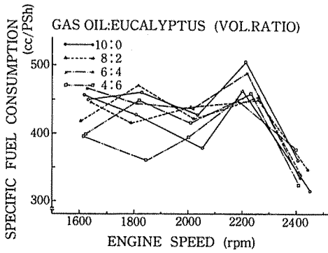
Fig. 9. — Specific fuel consumption curve
