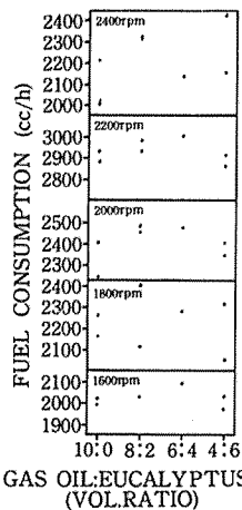
Fig. 8. — Relationships between blend ratio and fuel consumption
