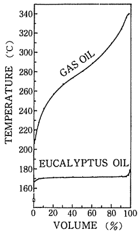
Fig. 1. - A.S.T.M. Distillation curve
