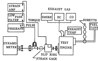
Fig. 2. Diagram of experiment apparatus
