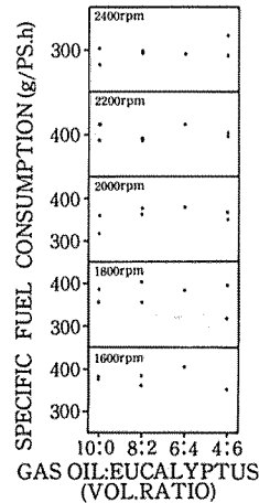
Fig. 12. — Relationships between blend ratio and specific fuel consumption
