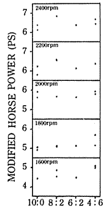
Fig. 4. — Relationships between blend ratio and modified horse power
