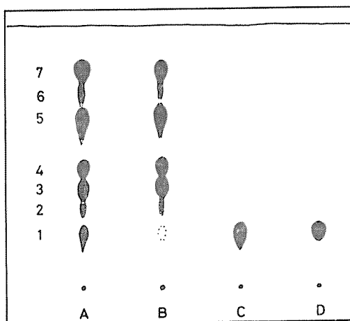
Fig. 1. Thin-layer chromatogram of waxes of the white variety of Koshu. Plate : Silicagel (Merk Art. 5721) activated at 110°C for 30 min., Solvent : Light petroleum (b. p. 60-70°C) : ether : acetic acid=70 : 30 : 1.5, Spray reagent : 5% K_2Cr_2O_7 in 40% H_2SO_4 and heating for 15 min. at about 200°C. A : total wax, B : soft wax, C : hard wax, D : authentic oleanolic acid. 1 : oleanolic acid, 2 and 3 : alcohols, 4 : acids, 5 : aldehydes, 6 : esters, 7 : hydrocarbons.
