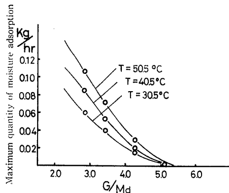
Fig. 9. Maximum quantity of moisture adsorption versus G/M_d in each air-temperature.
