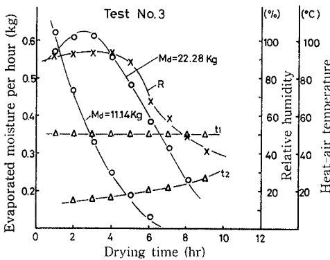
Fig. 4. Heat-air temperature = 50°C.
