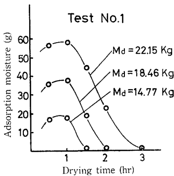
Fig. 6. Heat-air temperature = 30^{\circ}\text{C} .
