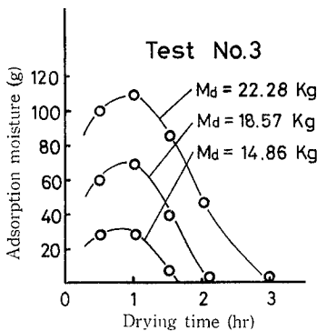
Fig. 8. Heat-air temperature = 50^{\circ}\text{C} .
