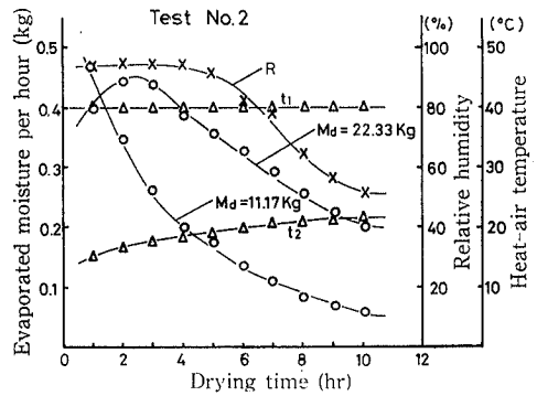
Fig. 3. Heat-air temperature = 40°C.
