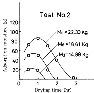
Fig. 7. Heat-air temperature = 40^{\circ}\text{C} .
