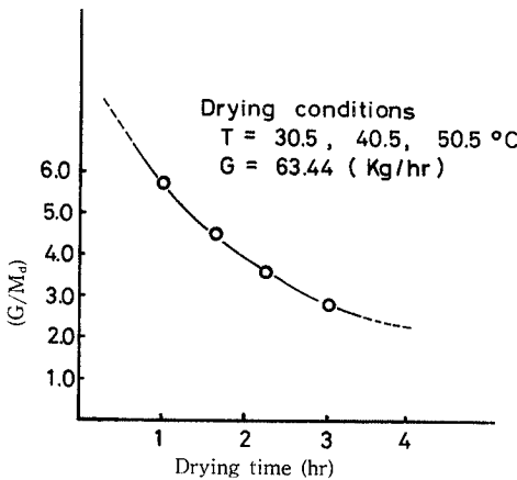
Fig. 11. Relation between the optimum (G/M_d) and drying hour in case of the deep-bed ventilation drying.
