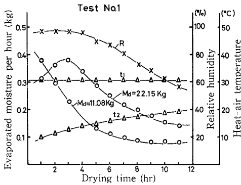
Fig. 2. Heat-air temperature = 30°C.
