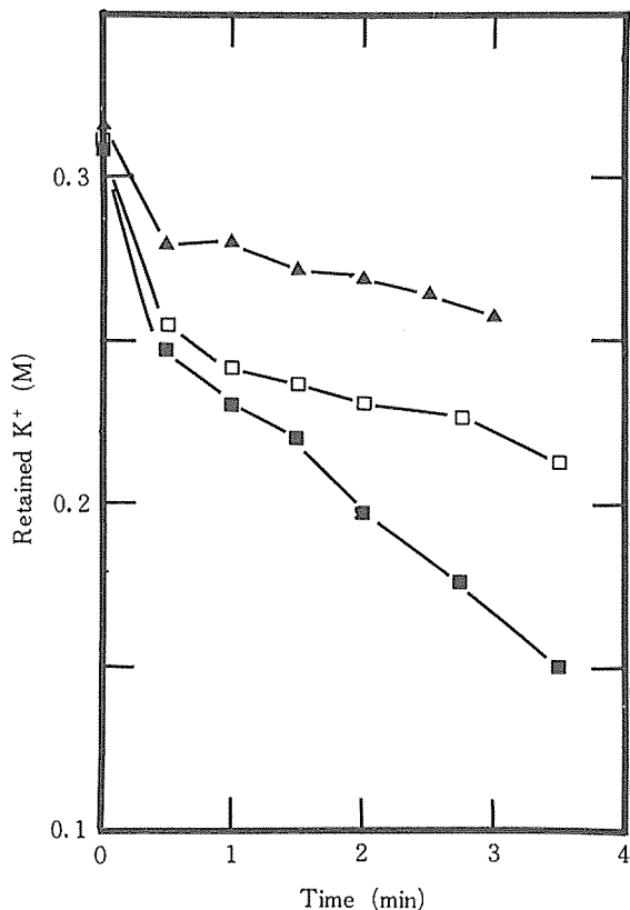
Fig. 3 Effect of H^+ -gradient on K^+ -release from K^+ -loaded vesicles.
