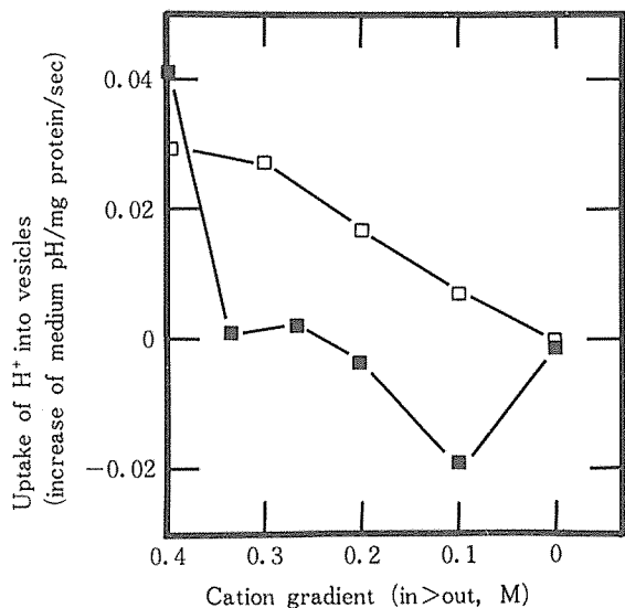
Fig. 2 Effect of K^+ - or Na^+ -gradient (in<out) on Na^+ -gradient (in>out) stimulated H^+ -uptake activity.
