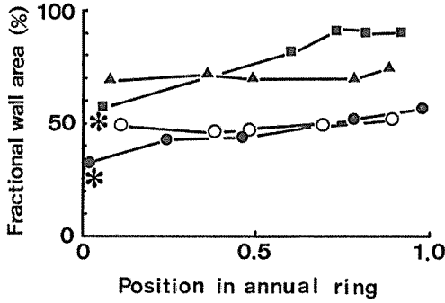
Fig. 8. Variation of fractional wall area of fibre within an annual ring. Note: ● kiri, ○ honoki, ▲ makanba, ■ kuri. * Vasicentric tracheids in kuri, axial parenchyma in kiri.
