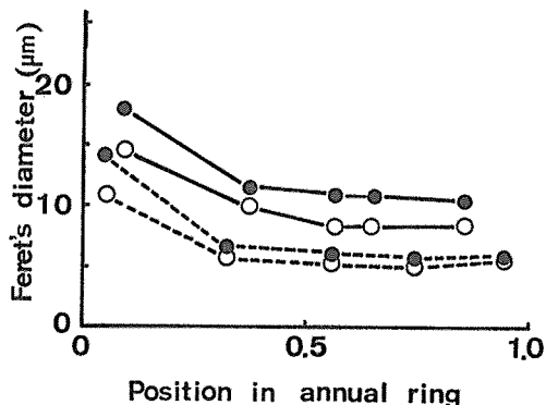
Fig. 3. Variation of Feret's diameter of fibre lumen within an annual ring in ring-porous wood (2). Note : ● radial diameter, ○ tangential diameter, — shioji, ..... keyaki.
