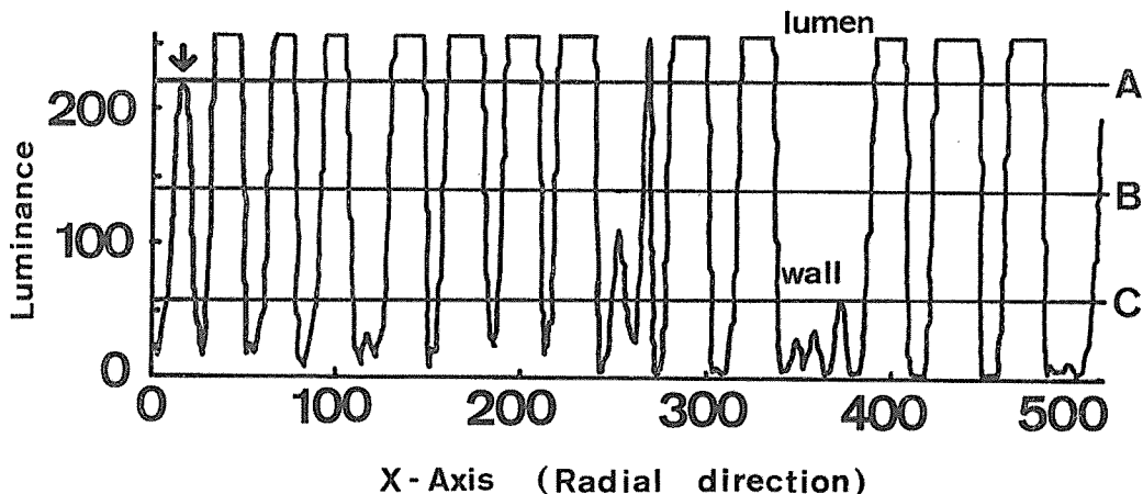
Fig. 1. Determination of threshold level on a profile of each sample section. Arrow indicates the luminance at the boundary between cell wall and lumen. Luminance : A < lumen, C > cell wall, B = threshold level (average value of A and C).
