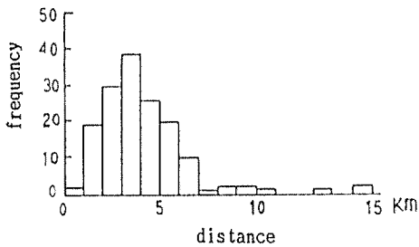
Fig. 5. Frequency distribution of the distance between each cellular echoes.
