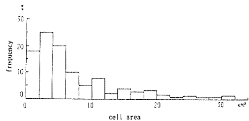
Fig. 3. Frequency distribution of rain cell area.
