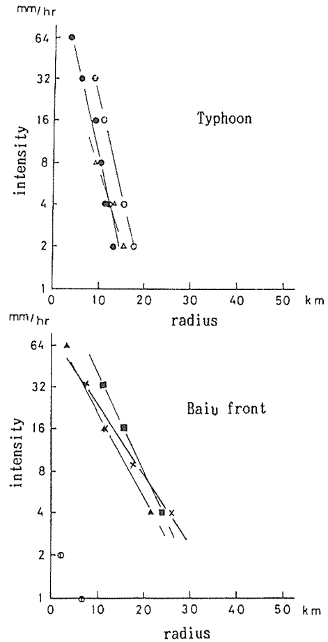
Fig. 9. Relations between rain intensity and cell area in case of Typhoon (upper) and Baiu front (lower).
