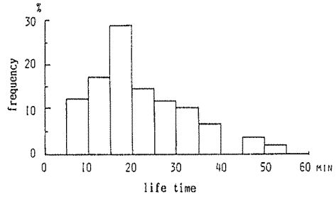
Fig. 6. Life line distribution of rain cells.
