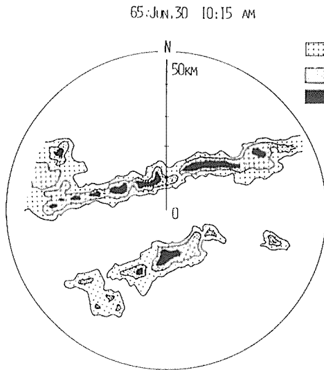
Fig. 1. Isohyetal map of radar echoes accompanied with Bain-front.
