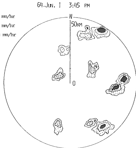
Fig. 2. Same as Fig. 1 accompanied with cumulonimbus.
