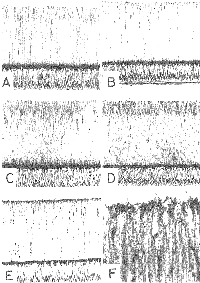
Fig. 2. Micrographs showing the migrating condition of the black pigment in retina of squids Sthenotiuthis oualaniensis (Lesson) when exposed to 100 V, 40 W lamps (see Fig. 7). (A) After 3 hours in darkness in the experimental tank. (B) Exposed 5 minutes. (C) Exposed 10 minutes. (D) Exposed 20 minutes, black pigment almost reach to the upper side of the retina. (E) Exposed 30 minutes, black pigment reach to the upper side of the retina. (F) Enlarged micrograph when the black pigment reached the upper side of the retina. Small black dotted point indicates black pigment. (A ~ E, \times 170 ; F, \times 850 ).
