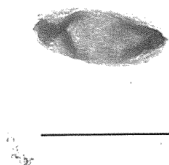
Fig. 1. Electron micrograph of Pseudomonas sp. 46NW-04 by negative stain with uranyl acetate.
