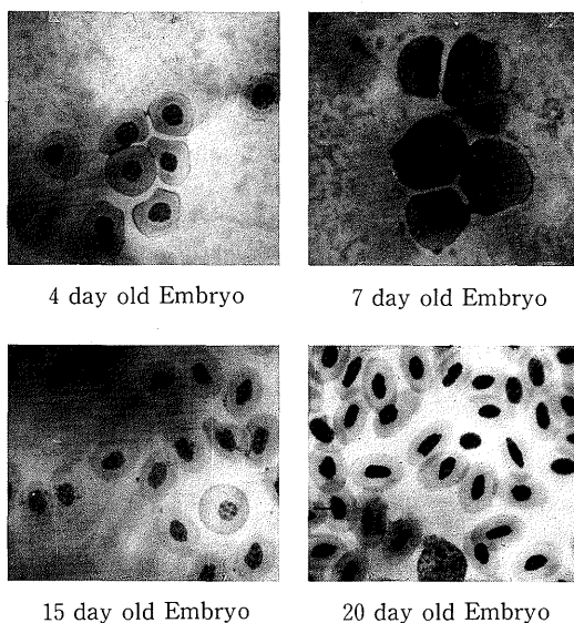
Fig. 1 Successive stages of erythrocyte development in chick embryos. ( \times 1,000 )
