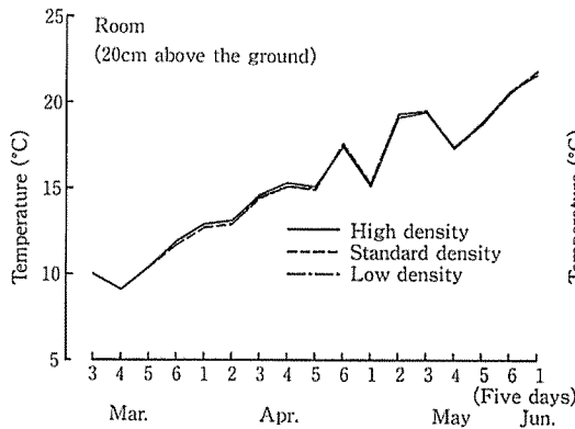
Fig. 3. Seasonal changes in room and soil temperatures (means of each 5 days).
