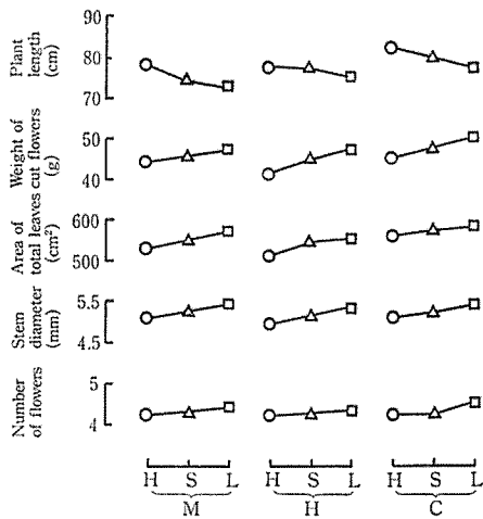
Fig. 5. Effect of the amount of applied organic fertilizer and plant density on the qualities of cut flowers of semi-forced lilies. H: high density, S: standard density, L: low density. M: much, H: half, C: control.
