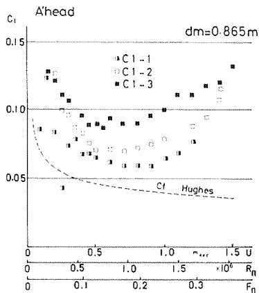
Fig. 3. Ahead resistance in ship loading conditions 1-1, 1-2, 1-3 ( C_1 = R_1 / (0.5 \rho S_w U^2) )
