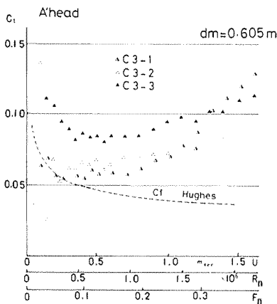
Fig. 5. Ahead resistance in ship loading conditions 3-1, 3-2, 3-3 ( C_1 = R_1 / (0.5 \rho S_w U^2) )
