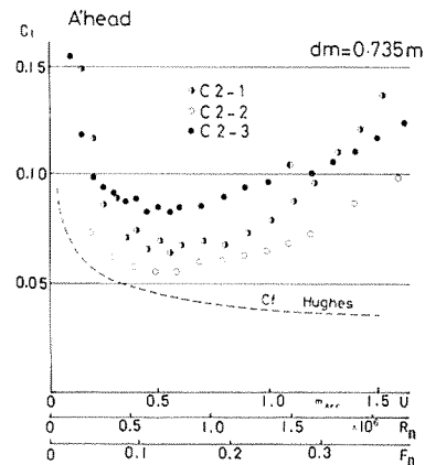
Fig. 4. Ahead resistance in ship loading conditions 2-1, 2-2, 2-3 ( C_1 = R_1 / (0.5 \rho S_w U^2) )
