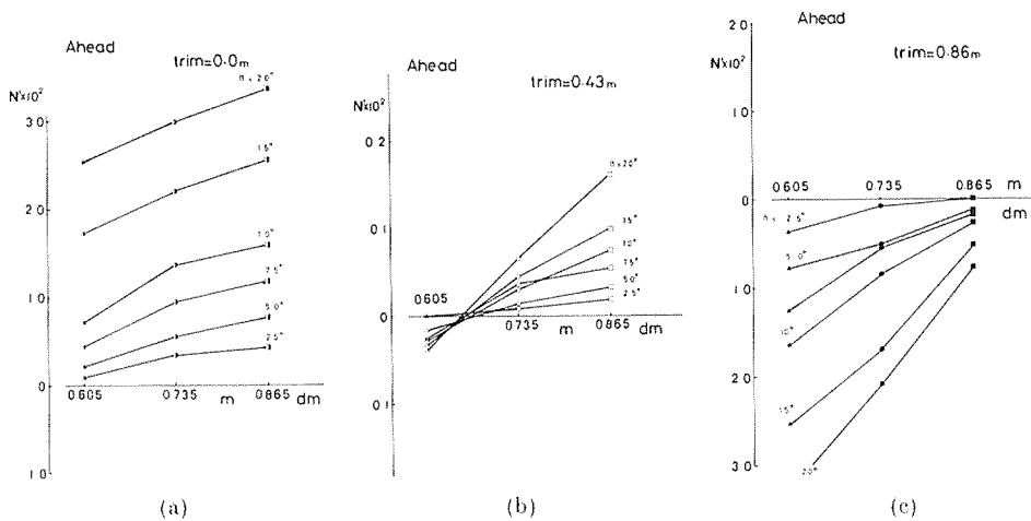
Fig. 8. The effects of draft conditions on nondimensional moment N'
