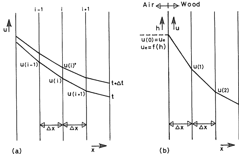
Fig. 1 Schematic diagram to explain a) diffusion of moisture through wood and b) boundary as wood surface equilibriate immediately with humidity of surrounding atmosphere.
