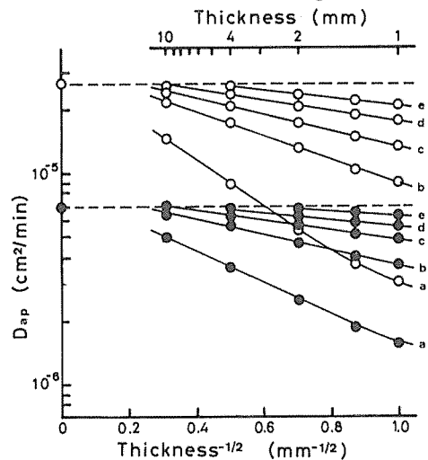
Fig. 5 Calculated apparent diffusion coefficient ( D_{ap} ) of wood at different surface transmission coefficient ( K ) and thickness.
