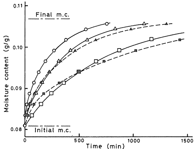
Fig. 6 Calculated adsorption processes (40% to 60% RH)
