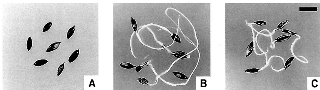
Fig. 2. Germination of Glehnia littoralis seeds promoted by cold stratification and the application of GA_3 . Seeds without treatment (A). Germination of seeds stratified at 5°C for 2 months (B). Seeds incubated at 20°C for 2 weeks in the presence of 10^{-3} M GA_3 (C). Scale bar indicates 1 cm.
