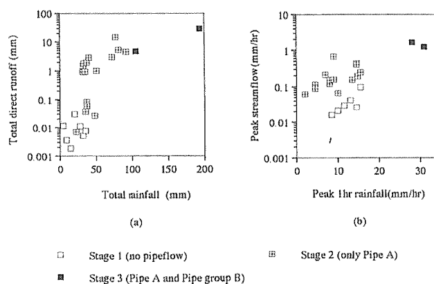
図-2 (a)総降雨量と総直接流量の関係および(b)ピーク1時間降雨強度とピーク1時間流域流量の関係（内田ら、1998b） Relationship between (a) the total rainfall and the total direct runoff, and (b) the peak 1 hour rainfall intensity and the peak 1 hour streamflow (after Uchida et al, 1998)
