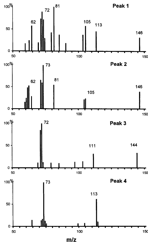
Fig. 2 Mass spectra of the four GC peaks. Peak 1: Diallyl Disulfide; Peak 2: C_6H_{10}S_2 ; Peak 3: 3-vinyl-[4H]-1,2-dithiin; Peak 4: Diallyl Sulfide.
