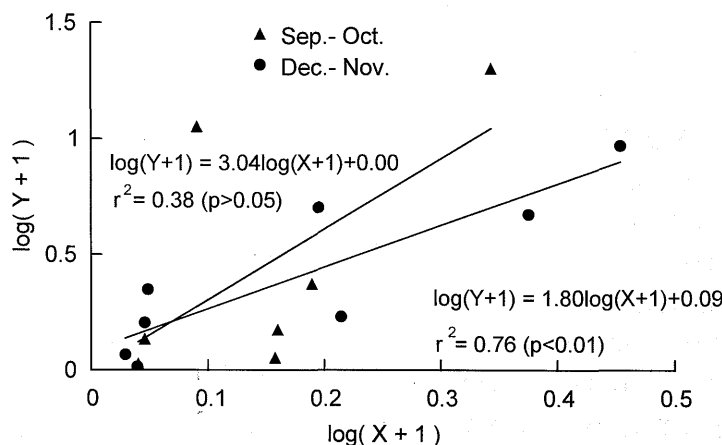
Fig. 17 Relationship between the number of adults captured per yellow sticky trap per day ( X ) and the number of larvae per plant ( Y ) of L. trifolii on tomatoes in experimental greenhouse. The number of larvae was counted 1 week after adult trapping. ▲: Date in Sep. and Oct. ●: Date in Dec. and Nov.
