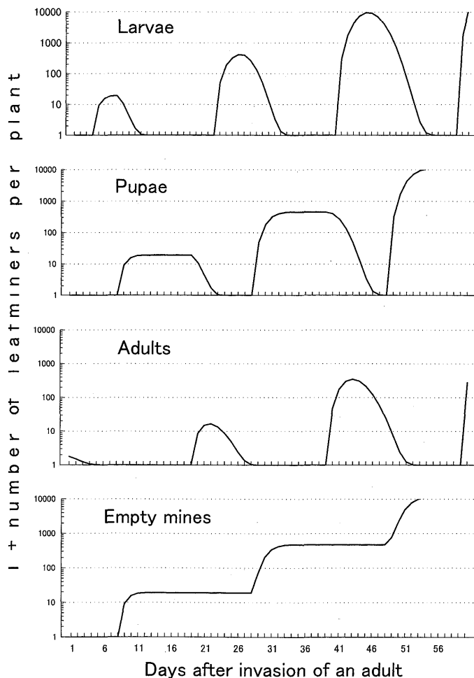
Fig. 5 Density of L. trifolii on tomato at 25°C predicted from the simulation model.
