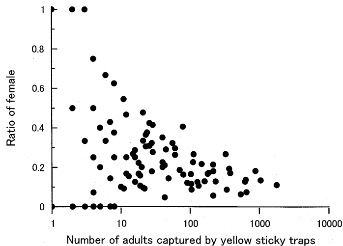
Fig. 14 Relationship between number of adults captured by yellow sticky traps and their sex ratio. A significant correlation was found by Spearman's rank correlation test ( r_s=0.31, p=0.01 ) using data with more than 9 adults.
