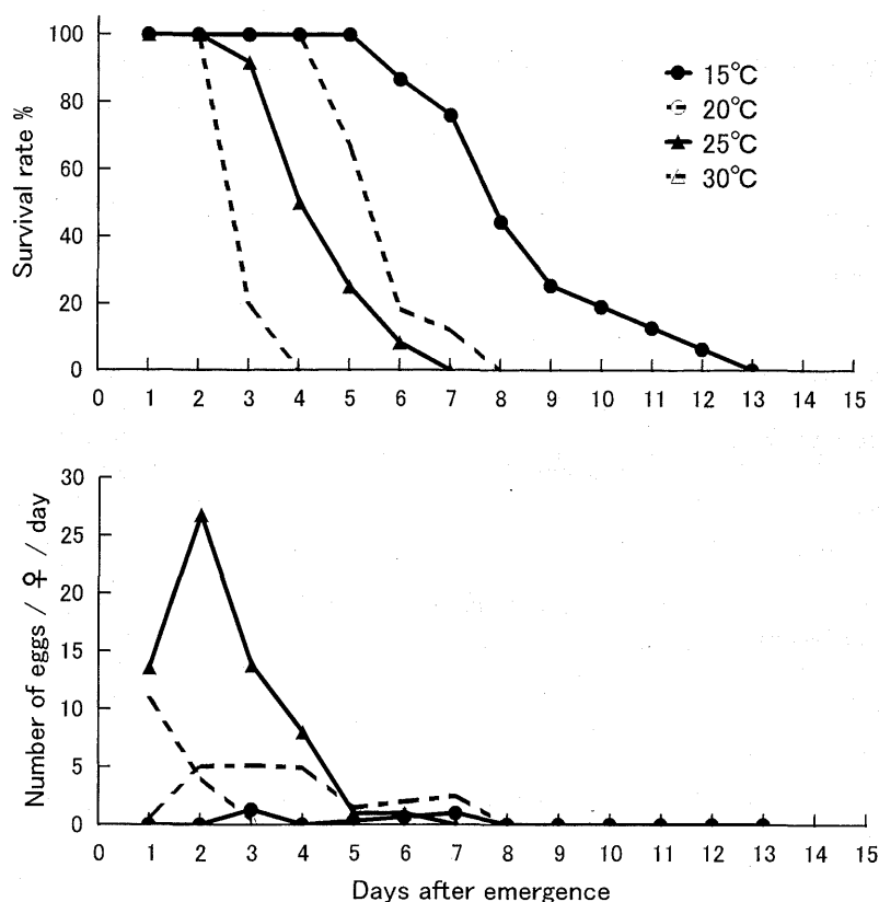
Fig. 4 Survival rate and daily egg production of L. trifolii females on tomato at different temperatures.
