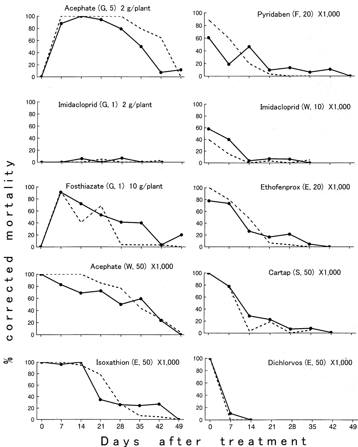
Fig.29 Residual contact toxicity of some insecticides on tomato leaves in greenhouse to adults of leafminer parasitoids, Diglyphus isaea and Dacnusa sibirica . Closed circles with solid line indicate D. isaea , open circles with broken line indicate D. sibirica . Formulation in parentheses, see Table 18.
