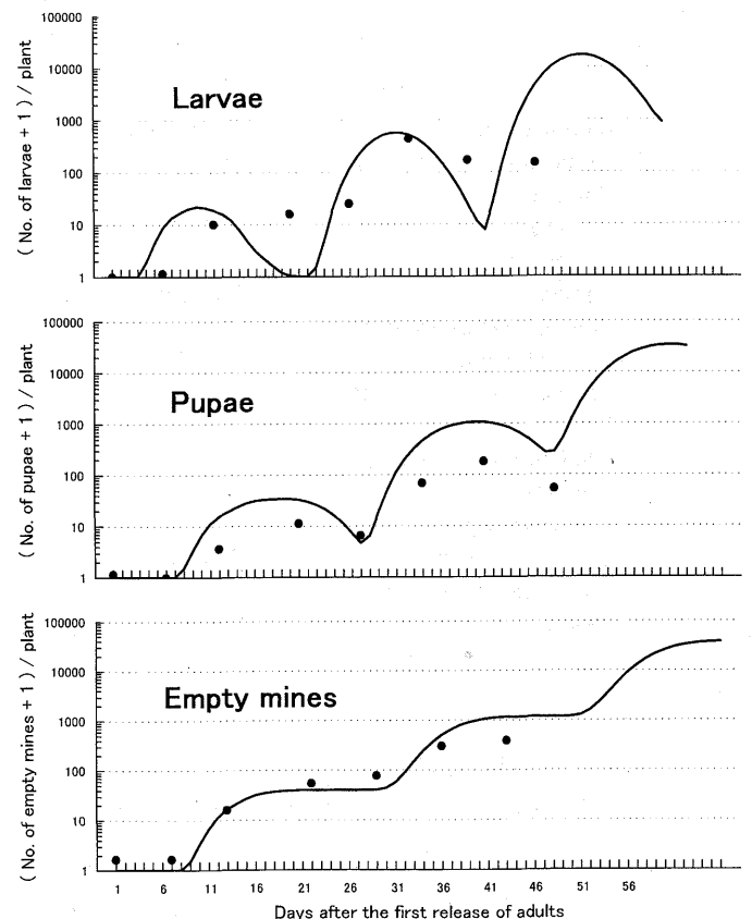
Fig. 6 Density of L. trifolii larvae, pupae and empty mines per plant predicted from the simulation model (solid lines) and those observed on tomatoes in the greenhouse (dots).
