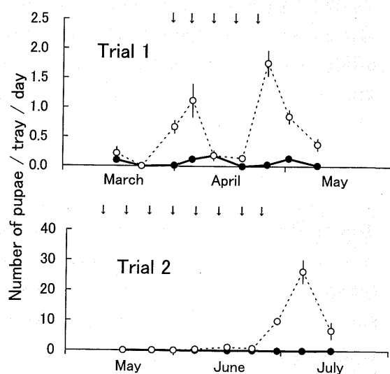
Fig.27 Number of L.trifolii pupae in trays under tomato plants in trials 1 and 2 (mean±SE). The symbols are the same as for Fig.24.
