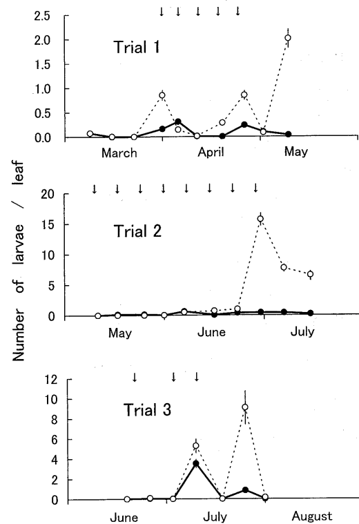
Fig.24 Number of L.trifolii larvae per leaf on tomato plants in trials 1,2 and 3 (mean \pm SE). Closed circles with solid line indicate data in greenhouse where Diglyphus isaea was released, open circles with dashed line indicate data in control greenhouse. Arrows show the timing of parasitoid releases.
