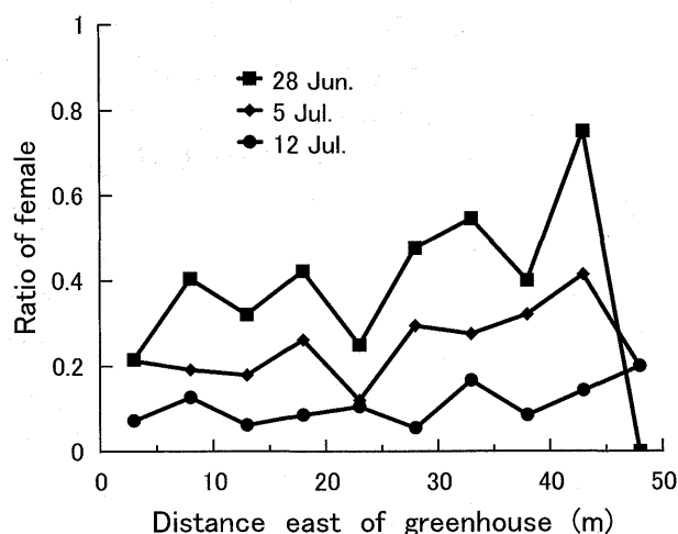
Fig. 13 Sex ratio of adults captured by yellow sticky traps placed horizontally in row.
