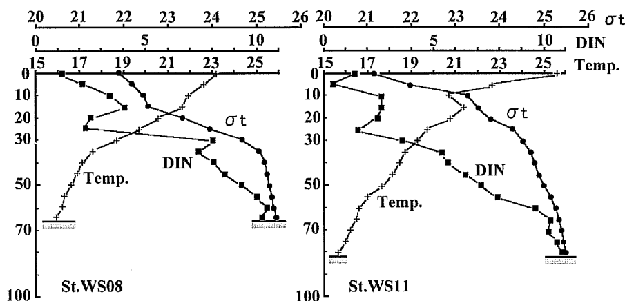
Fig. 5-33. Vertical profiles of temperature (+ marks: in ^{\circ}\text{C} ), sigma-t (black circles), and DIN (black squares: in \mu\text{g-at/l} ) at WS08 (left figure) and WS11 (right figure) on August 2, 1995.
