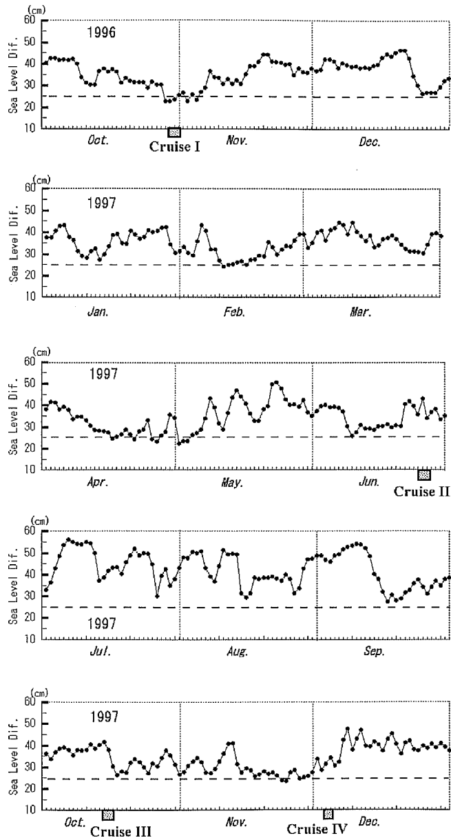
Fig. 3-28. Variation of the daily averaged value of the sea level difference between Kushimoto and Uragami for the period from October 1996 to December 1997. The horizontal dashed line at 25 cm difference in the figure is the threshold value whether the Kuroshio has the straight path or the large meandering path. The straight path usually occurs if the difference is larger than 25 cm, and the meandering path occurs if it is near or smaller than 25 cm (Fujita 1997). The periods of the four cruises are indicated with bold bars under the column.
