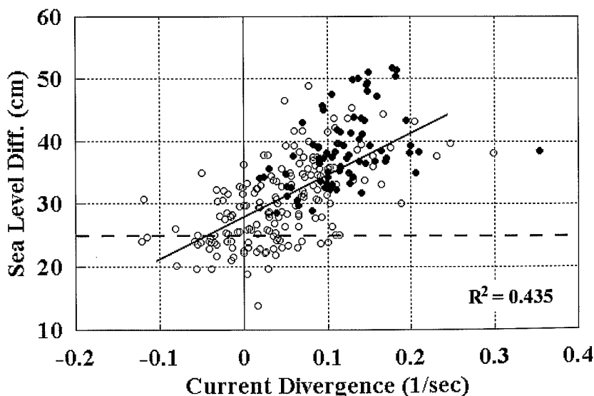
Fig. 3-18. Correlation between the daily average value the sea level difference between Kushimoto and Uragami and the current divergence averaged over the central portion of the standard line (Fig. 3-16). Black dots indicate the case of the Typical Bifurcation Current. White dots indicate the other Current pattern which the other Bifurcation Current, the Eastward Current, the Westward Current, the Converging Current, and the Irregular Current.
