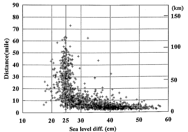
Fig. 3-6. Correlation between the positions of the Kuroshio axis measured due southward from Cape Shionomisaki (in mile and km) and the sea level difference between Kushimoto and Urakami (in cm) during January 1999 to December 2003. The distance was determined from satellite image of surface temperature distribution by the Marine Fisheries Experimental Station, Wakayama Research Center of Agriculture, Forestry and Fisheries, and the sea level difference averaged for each day is used.
