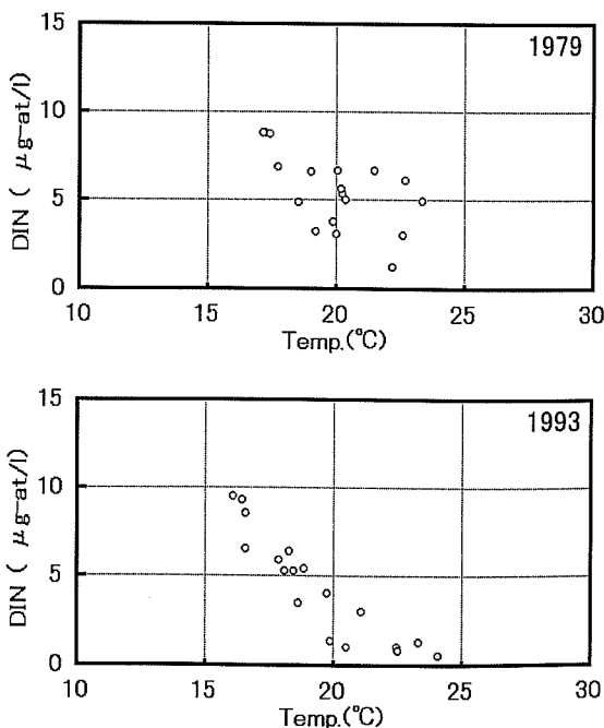
Fig. 5-27. Same as in Fig. 5-24, except for in August 1979 (upper figure) and for in August 1993 (lower figure).
