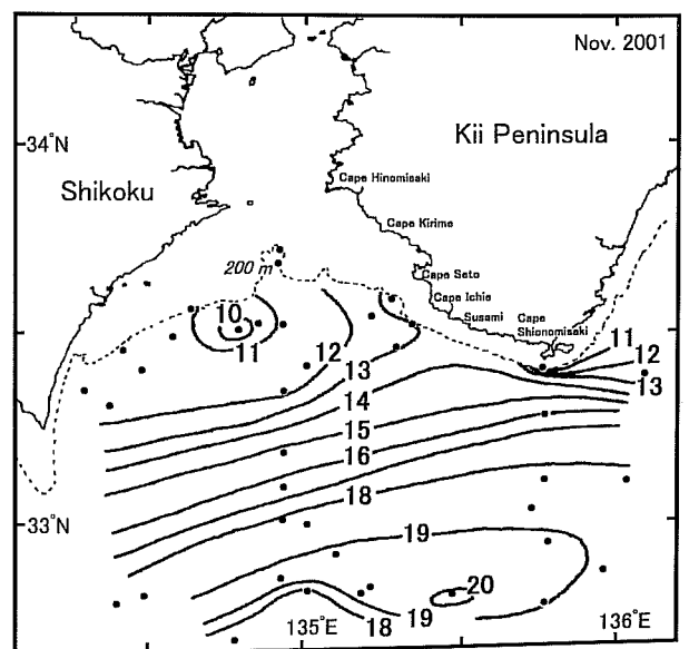
Fig. 5-4. Horizontal distribution of the water temperature at 200m depth based on data taken in the period from November 12 to 18, 2001. Numerals attached to isotherms show temperature in °C. Positions of observation points are given by black dots.
