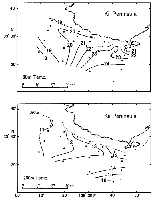
Fig. 3-30. Temperature distributions at the depths of 50 m (upper figure) and 200 m (lower figure) in the period from June 24 to June 25 (Cruise II). Dots in the figure indicate the position of the XBT observations.
