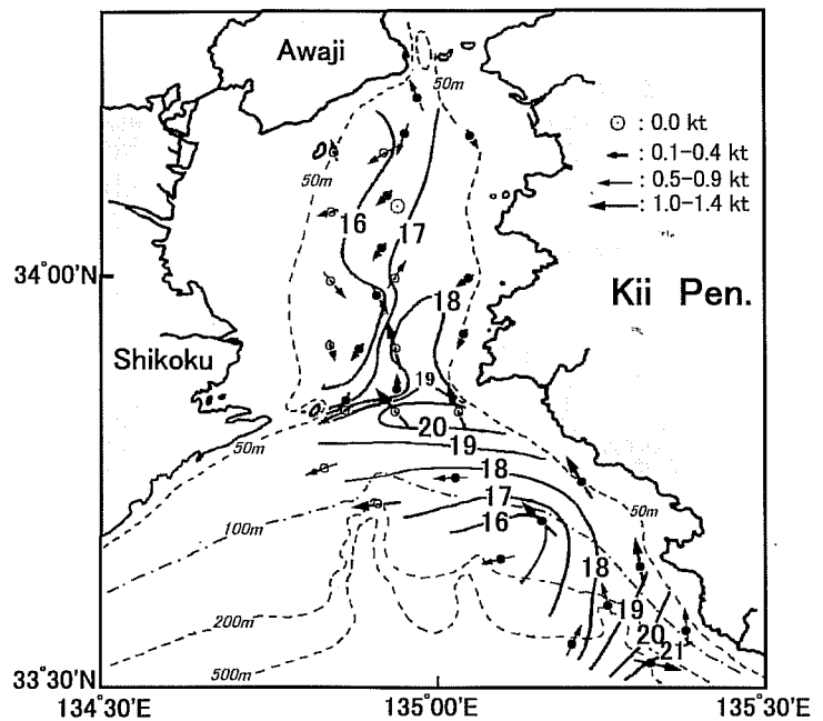
Fig. 5-20. Temperature distribution at the depth of 50m on August 1-4, 1995. Numerals attached to isotherms indicate temperature in ^{\circ}\text{C} . Current velocities at 5m depth measured with ADCP are shown as arrows. Scale of the current velocity is shown in right top in the figure. Dashed lines also show bottom contours for 50m, 100m, 200m, and 500m.
