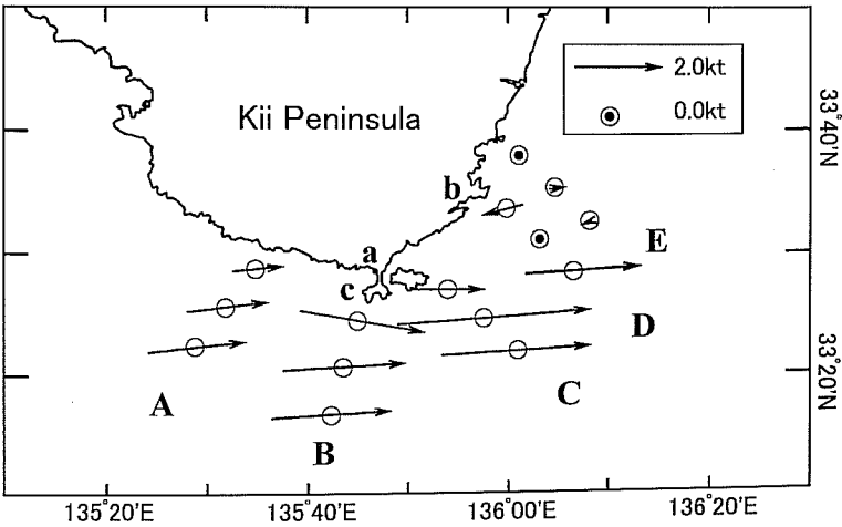
Fig. 3-3. Surface current field (5 m) measured by ADCP of the R/V Wakayama on June 11-12, 1996. a indicates the position of the Kushimoto tide gauge station, b that of the Uragsami tide gauge station, and c Cape Shiono-misaki.
