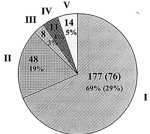
Fig. 3-13. Occurrence frequency of each flow pattern; I: the Bifurcation Current, II: the Eastward Current, III: the Westward Current, IV: the Converging Current and V: the Irregular Current. The occurrence frequencies are given both by number and by % are shown in each corresponding section (numbers in parenthesis indicate the Typical Bifurcation Current).
