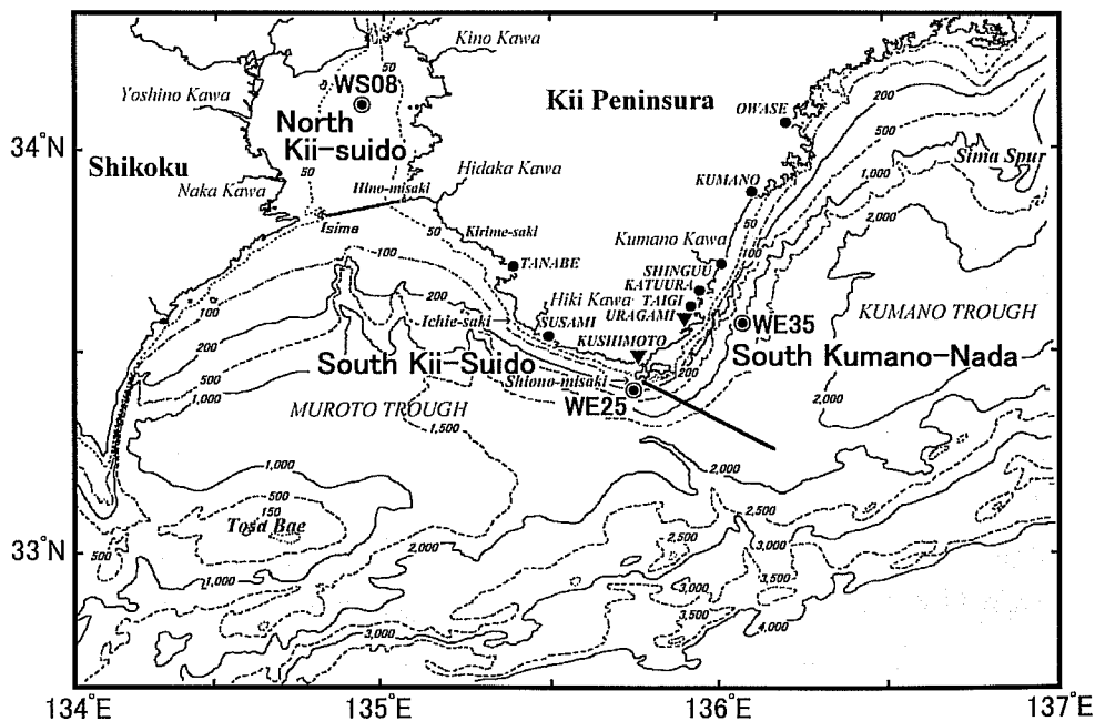
Fig. 1-1. Location of the study area in this paper. The area is divided into the southern Kumano-nada, the southern Kii Channel, and northern Kii Channel. Locations of observation points, WS08, WE25 and WE35 which are selected as representative points for the northern Kii Channel, the southern Kii Channel and the southern Kumano-nada, respectively. The locations of two tide gauge stations at Kushimoto and at Urugami are shown with ▼. Bottom topography is shown. Numerals attached to bottom contours indicate depth in m. Locations of main rivers, of main capes, and of main cities and towns are given.
