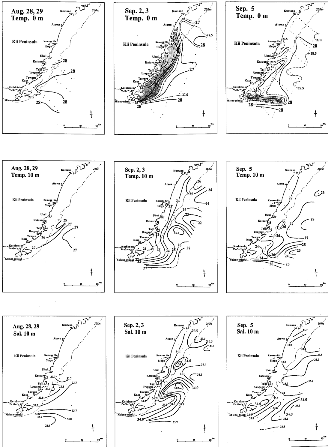
Fig. 4-16. Variations of horizontal temperature fields at the sea surface (upper figures), and at 10m depth (middle figures), and horizontal salinity field at 10m depth (lower figure). Distributions observed on August 28-29, September 2-3, and September 5, 1985 are shown in left, middle, and right panels, respectively. Numerals attached to isotherms indicate temperature in °C, and those attached to salinity isopleths indicate salinity in psu units. The area where surface temperature is below 26°C is shaded in the upper figures.
