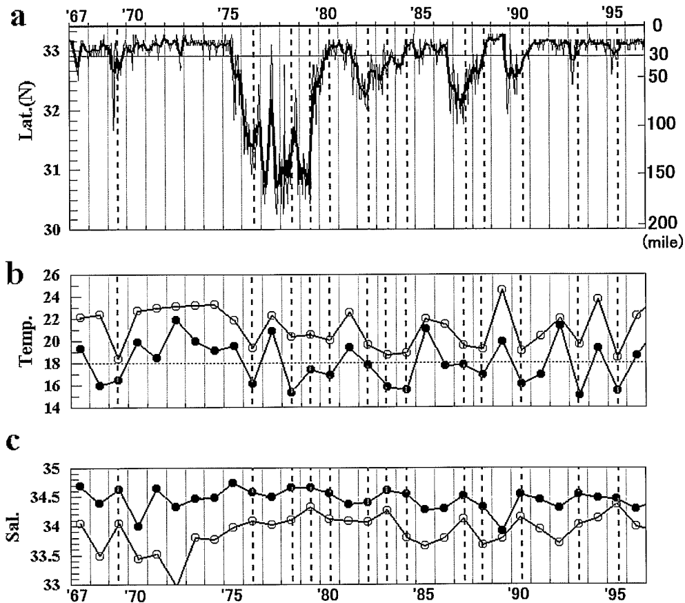
Fig. 5-16. Temporal variations in the period from 1967 to 1996 of the distance (in nautical miles) of the Kuroshio axis, which was measured southward from Cape Shionomisaki (a), of averaged temperature for July, August and September data of each year (white circles) and of the minimum temperature among three months (black circles) measured at 50m depth of SW08 (b), and of averaged and the maximum salinity obtained by the same manner (c). The distance of the Kuroshio axis was determined from the Prompt Report of Oceanographic Conditions published bimonthly by the Hydrographic and Oceanographic Department, Japan Coast Guard. The values plotted here are bimonthly data (thin line) and 2.5 months running mean (bold line) in the top figure. Distance of 30 nautical mile is shown with a horizontal line. The horizontal dotted line in the middle figure shows 18°C. The typical cold bottom water is defined when the minimum temperature is below this temperature. Vertical dashed lines indicate the occurrence years of cold bottom water, except for 1968, 1986 and 1991 when low salinity values were observed.
