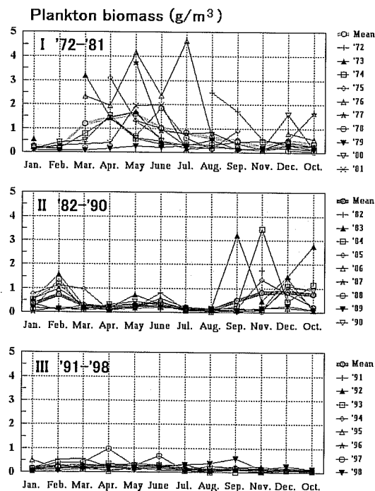
Fig. 5-37. Seasonal variation of plankton biomass (in \text{g/m}^3 ) for each year. The variations are shown for period I (1972-1981: upper figure), for period II (1982-1990: middle figure) and period III (1991-1998). Identification of the year is given with symbols as shown on the right of each figure.
