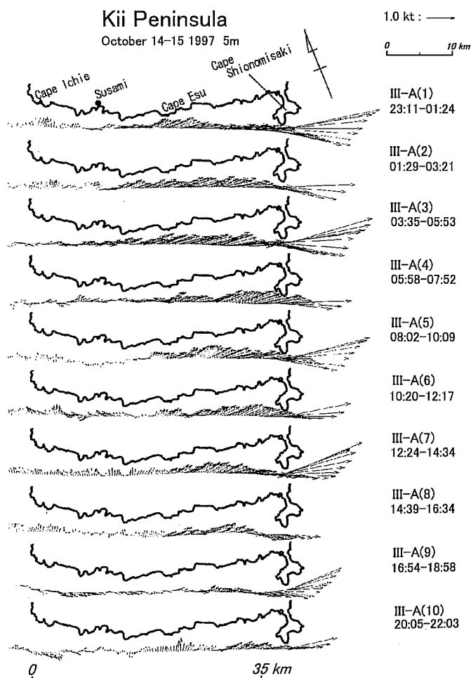
Fig. 3-39. Same as in Fig. 3-32 except at 5 m depth for 10 repeated runs in Cruise III.
