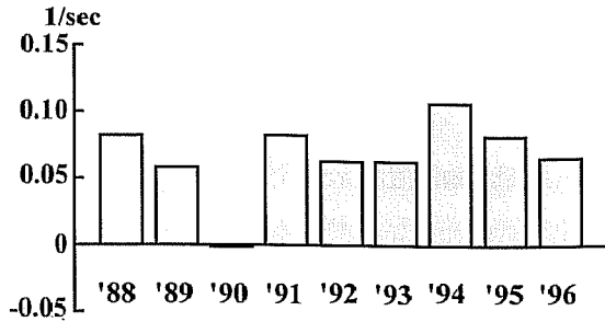
Fig. 3-20. Temporal variation of the current divergence (in 1/sec) yearly averaged over the standard line.
