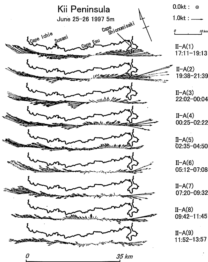
Fig. 3-32. Current field of each repeated run of Cruise II at 5 m depth. The observation period of each run is shown in the rightmost portion of each row of the figure. The bold horizontal line at the bottom of the figures indicates the position where the current divergence was averaged (Table 3-4 and Fig. 3-44 a). The time required to carry out each repeated line is usually less than 2 hours, and tidal currents appear not to influence the flow pattern. The magnitude of the current vector is indicated at the right-upper corner of the figure.
