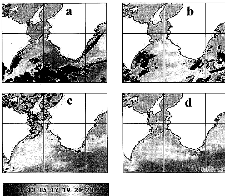
Fig. 5-13. Satellite images of sea surface temperature data source from AGROPEDIA of the Agriculture, Forestry and Fisheries Research Center. (a) April 21-22, (b) April 24-25, (c) April 26-27, and (d) April 28-29, 1994. Correspondence of color to brightness temperature is shown below the figures.
