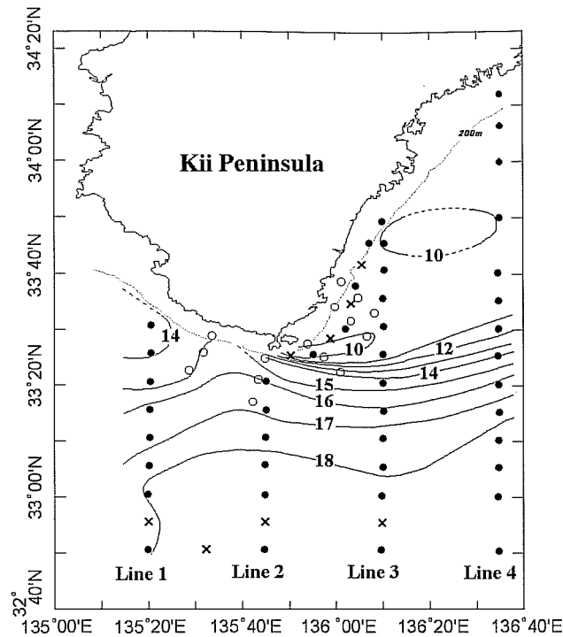
Fig. 3-1. Observation sites of the R/V Seisui-maru of Mie University on June 11-14, 1996 and of the R/V Wakayama of the Fisheries Experimental Station, Wakayama Research Center of Agriculture, Forestry and Fisheries on June 11-12. The CTD observation points by the R/V Seisui-maru and by the R/V Wakayama are indicated with black circles and white circles, respectively, and the XBT observation points by R/V Seisui-maru with x. The horizontal temperature distribution at the depth of 200 m (in °C) is also shown.
