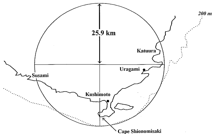
Fig. 3-4. Coastline and 200 m bottom contour in the vicinity of Cape Shionomisaki. The bottom contour just to the south and to the east is approximated by a circle (drawn in bold in the figure: the radius of the circle is 25.9 km). Black dots indicate the positions of two tide gauge stations, Kushimoto and Urugami. The sea level difference between these two stations is used to monitor the states of the Kuroshio path, namely in a straight path or a meandering path.
