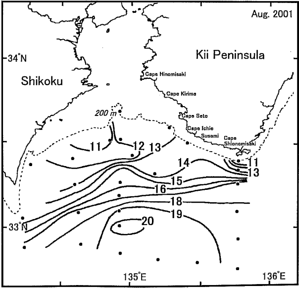
Fig. 5-9. Same as in Fig. 5-4, except for the period from August 24 to 30, 2001.
