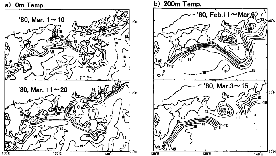
Fig. 4-11. Surface temperature distributions based on data taken in the period from March 1 to 10, 1980 (upper left figure) and based on data taken in the period from March 11 to 20, 1980 (lower left figure) after the Japan Fisheries Information Center, and temperature distribution at 200m depth based on data taken in the period from February 11 to March 6, 1980 (upper right) and based on data taken in the period March 3 to 15, 1980 (lower right figure) after the Prompt Report of Oceanographic Conditions published bimonthly by the Hydrographic and Oceanographic Department, Japan Coast Guard. Numerals attached to isotherms indicate temperature in °C. w and c show relatively high and low temperature portions, respectively.
