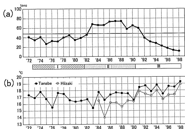
Fig. 5-42. Variation of the yearly catch of abalones reported by 5 fisheries co-operative associations near Cape Hinomisaki is shown in upper figure (a). The averaged surface temperature for the period from November to next February in Tanabe Bay (black circles), and that at Hiizaki (white circles) are shown in lower figure (b). See Fig. 5-43 for these locations. Periods I, II, and III are shown at the bottom of the upper figure. Horizontal bold line in upper figure indicates the averaged yearly catch in the period from 1972 to 1998.
