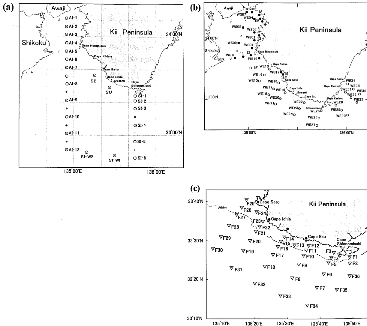
Fig. 5-1. Station maps of the routine observations carried out by the Marine Fisheries Experimental Station, Wakayama Research Center of Agriculture, Forestry and Fisheries (renamed from the Wakayama Prefectural Fisheries Experimental Station). (a) Stations of the offshore lines: white circles indicates CTD stations, x XBT stations, and + surface water sampling stations. Station name is attached to each CTD station. A CTD station between AI-7 and AI-8 is occupied optionally and no name is given. AI and SI are the line names. (b) Stations of the coastal lines (white circles) and shallow water lines (black circles), respectively. Numeral attached to each station is the station number, and WS is attached before the station number for the shallow water stations and WE for the coastal stations number, respectively. The station WE-15' is an additional station at the time of high frequency survey conducted in 1995. (c) Stations adapted in the high frequency survey conducted in July 25-26 and in August 24, 1995.
