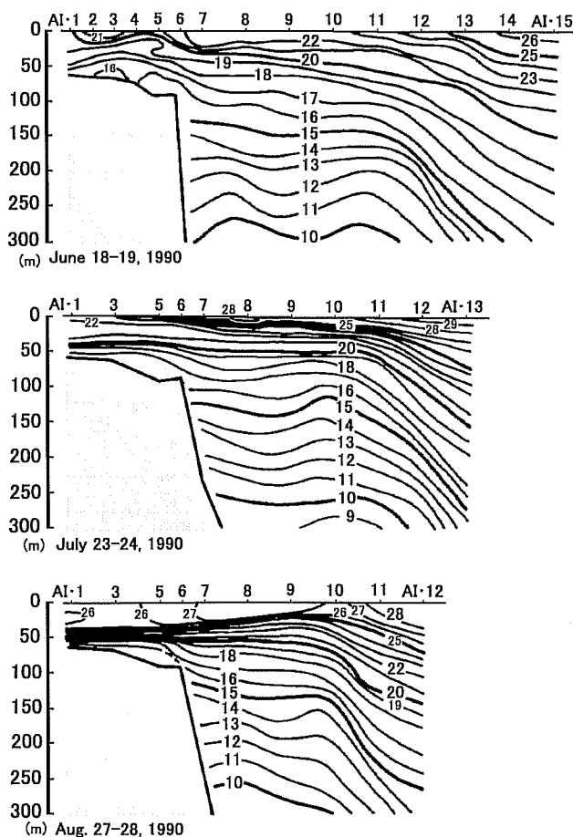
Fig. 5-22. Temperature cross-sections along AI line on June 18-19 (upper figure), on July 23-24 (middle figure), and on August 27-28, 1990. Numerals attached to isotherms indicate temperature in °C.
