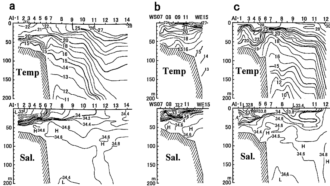
Fig. 5-18. Temperature (upper figures) and salinity (lower figures) cross-sections along AI line on July 18-19 (a), along line B on August 1-2 (b), and along AI line on August 21-22 (c), 1995. The positions of the lines AI and B are shown in Fig. 5-19. Numerals attached to isopleths in the figures indicate temperature in 1 °C (upper figures), and salinity in psu (lower figures), respectively. Station names are given in the upper margin of the figures.
