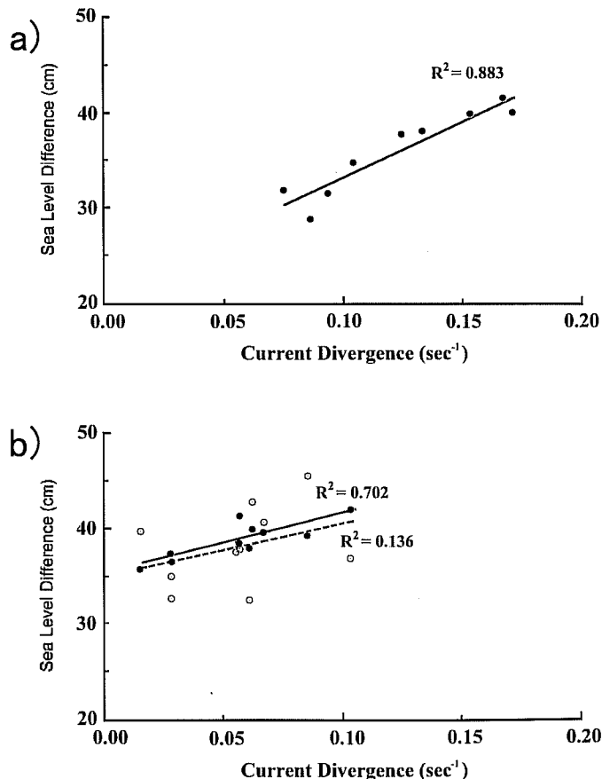
Fig. 3-44. Correlation between the hourly value the sea level difference between Kushimoto and Uragami and the current divergence averaged over the central portion of the standard line. a) At the time of the repeated runs in Cruise II. The regression line is shown with a full line and the square of the correlation coefficient is shown in the figure. b) At the time of the repeated runs in Cruise III: white dots indicate the case that the raw value of the sea level difference is taken in the ordinate, and black dots the case that the sea level difference has been used after elimination of the tidal signal (see Fig. 3-38). The regression lines are shown as a dashed line ( R^2=0.136 ) and a full line ( R^2=0.702 ), respectively.
