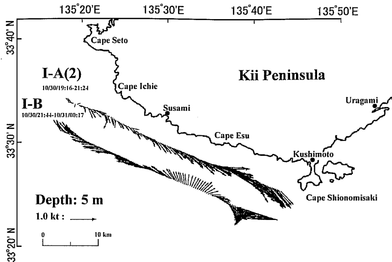
Fig. 3-37. Horizontal distribution of the current in I-A(2) and I-B in Cruise I. The magnitude of the current vector is indicated at the left-lower corner of the figure (in \text{kt} = 0.5 \text{ m/s} ).
