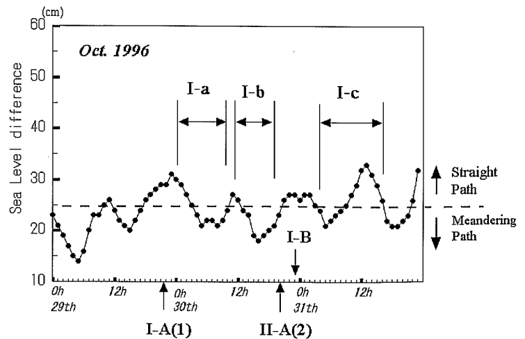
Fig. 3-34. Same as in Fig. 3-31 except for Cruise I.
