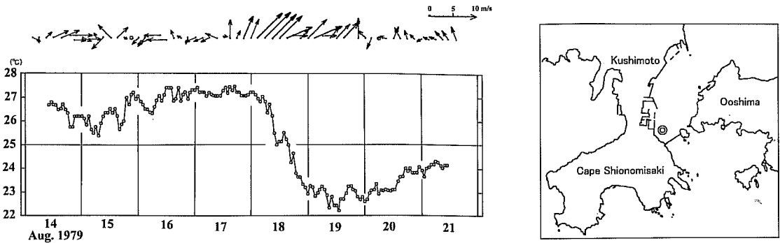
Fig. 4-22. Variation of temperature at 10m depth at the fish farm buoy station, (see right figure for its location; ◎) in the period from August 14 to 21, 1979. Variation of three hourly interval wind velocity at Cape Shionomisaki is shown above the figure. Scale of wind speed is given at the right upper corner.
