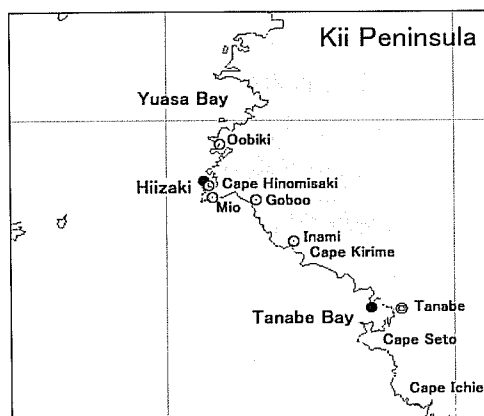
Fig. 5-43. Locations of Cape Hinomisaki, Tanabe Bay and Yuasa Bay. Positions of temperature measurement in Tanabe Bay and at Hiizaki are shown as black circles. Locations of Fisheries Co-operative Associations (Oobiki, Hiizaki, Goboo, Inami) are shown with white circles.
