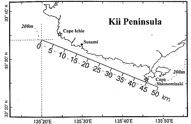
Fig. 3-16. The standard line where the current divergence was determined.
