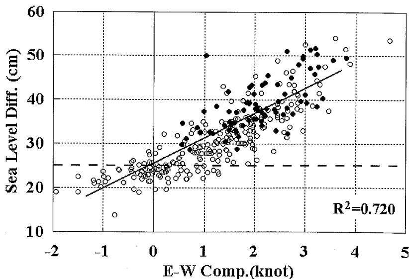
Fig. 3-26. Correlation between the daily average value of the sea level difference between Kushimoto and Urugami and the current velocity in the vicinity of Cape Shionomisaki, where locate the east area of the Bifurcation Current. Black dots indicate the case of the Typical Bifurcation Current. White dots indicate the other Current pattern which the other Bifurcation Current, the Eastward Current, the Westward Current, the Converging Current, and the Irregular Current.
