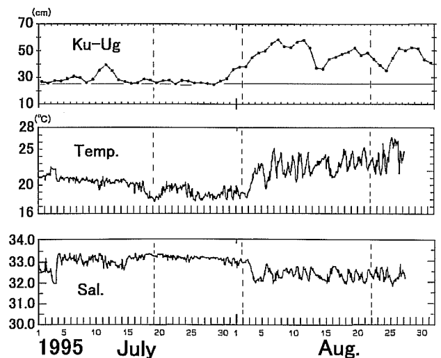
Fig. 5-21. Temporal variations of sea level difference between Kushimoto and Urugami tide gauge stations (upper figure), and of temperature (middle figure) and salinity (lower figure) at 30m depth of Station K5 in the period from July 1 to August 31, 1995. Nominal observed value at Kushimoto is subtracted by that at Urugami for sea level difference. Vertical dashed lines indicate the times when the cross-sectional distributions in Fig. 5-18 were observed.
