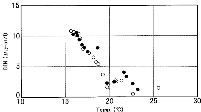
Fig. 5-34. Relations between temperature and DIN at WS08 (black circles) and WS11 (white circles). See Fig. 5-33 for their vertical profiles.
