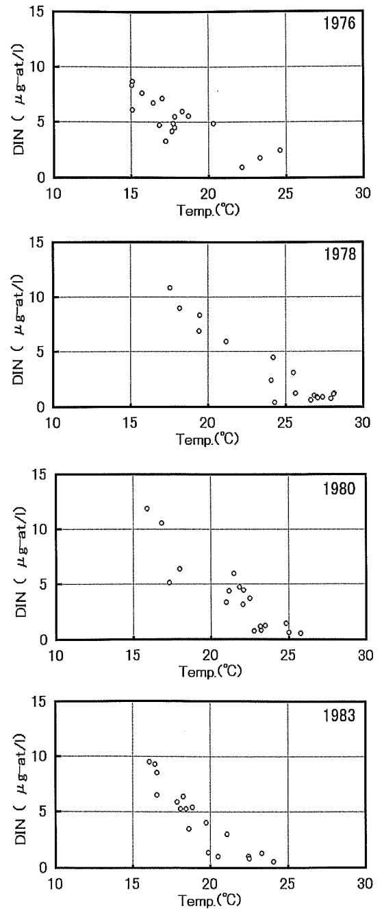
Fig. 5-26. Same as in Fig. 5-24, except for in August 1976, in August 1978, in September 1980, and in August 1983 from top to bottom.
