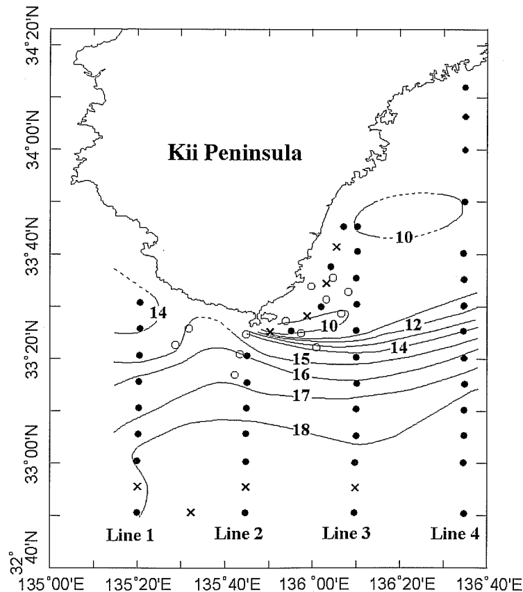
Fig. 3-27. Observation sites of the R/V Seisui-maru of Mie University on June 11-14, 1996 and of the R/V Wakayama of the Wakayama Research Center of Agriculture, Forestry and Fisheries, Marine Fisheries Experimental Station on June 11-12. The CTD observation points by the R/V Seisui-maru and by the R/V Wakayama are indicated with black circles and white circles, respectively, and the XBT observation points by R/V Seisui-maru with x. The horizontal temperature distribution at the depth of 200 m (in °C) is also shown.
