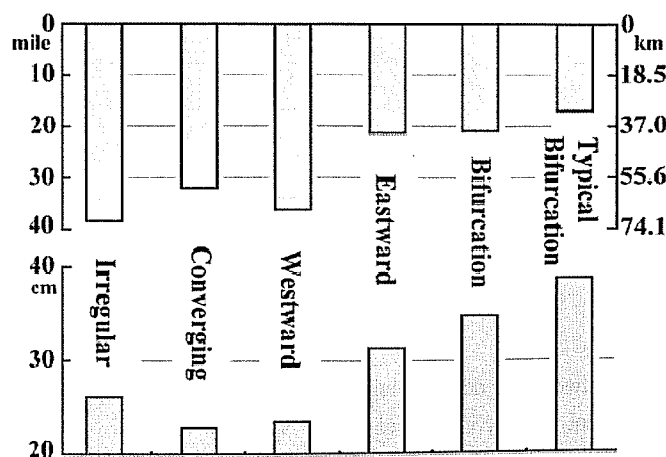
Fig. 3-25. Position of the Kuroshio axis measured southward from Cape Shionomisaki and the sea level difference between Kushimoto and Uragami for each current pattern.
