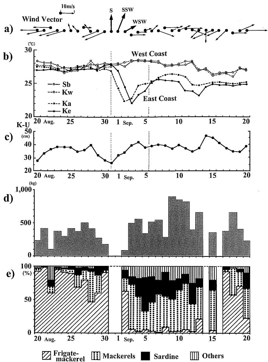
Fig. 4-15. Daily maximum instantaneous wind velocity ( a : scale of wind speed is shown right upper), of surface temperatures ( b : in °C) at four routine surface temperature observation points, Sabura (Sb), Kushimoto west coast (Kw), Kushimoto east coast (Ke), and Katsuura (Ka) (see Fig. 4-13 for their locations: Sb and Kw are located to the west of Cape Shionomisaki, and Ke and Ka to the east of Cape Shionomisaki), at 9:00 a.m., of sea level difference ( c : in cm) between Kushimoto and Uragami tide gauge stations (the nominal sea level value at Kushimoto is subtracted by that at Uragami), of daily catch ( d : in kg/boat/day) and species constitution ( e : in %: classification of species is shown below the figure) by stick-held dip net boats belonging to the Katsuura Fisheries Co-operative Association.
