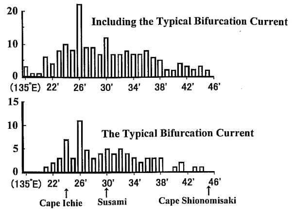
Fig. 3-14. The frequency histograms against the position (in longitude) are shown for both the Bifurcation Current (upper figure: including the Typical Bifurcation Current) and the Typical Bifurcation Current only (lower figure). Two figures show an almost identical shape, and the weak peak of bifurcation point appears near Cape Ichie in each curve.
