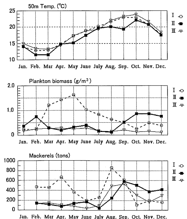
Fig. 5-39. Seasonal variations of temperature measured at 50m depth of WS08 (upper figure, in °C), of plankton biomass (middle figure, in g/m³), and of the mackerels catch (lower figure, in tons). Monthly averaged values are given for period I (white circles connected with dashed line), for period II (black squares connected with bold line), and for period III (white triangles connected with thin line).
