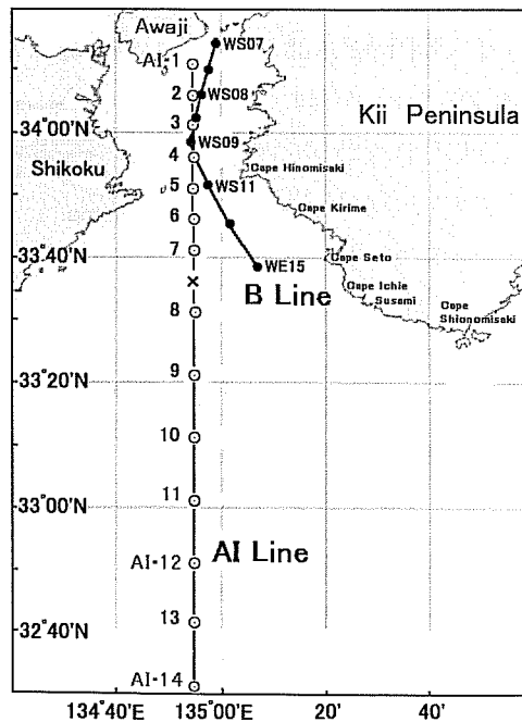
Fig. 5-19. Locations of AI line and B line, along which cross-sectional distribution of temperature and salinity are given in Fig. 5-18. x mark along AI line indicates the position of XBT observation. CTD observations were made at other stations.
