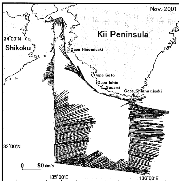
Fig. 5-3. Horizontal distribution of current velocity on 17m depth surface, which was observed with ADCP by the Marine Fisheries Experimental Station, Wakayama Research Center of Agriculture, Forestry and Fisheries in the period from November 20 to 21, 2001. The scale of velocity vector is given near the left bottom corner.
