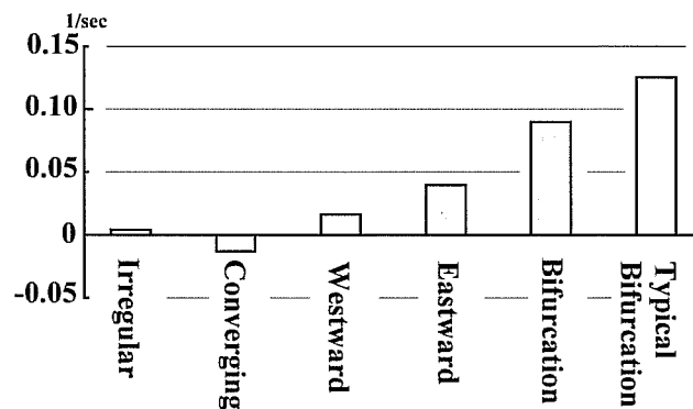
Fig. 3-24. Current divergence averaged for each flow pattern.
