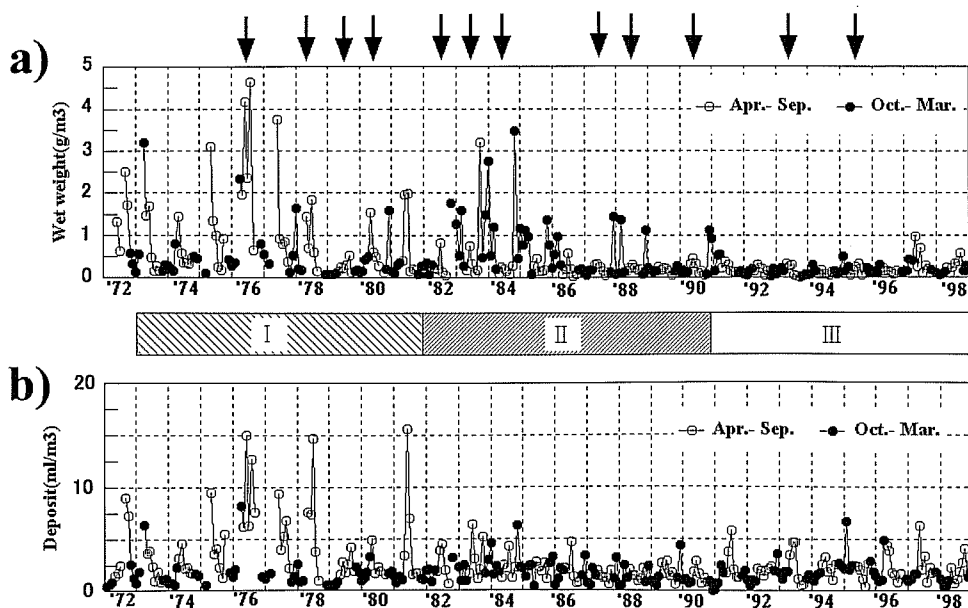
Fig. 5-36. Temporal variations of plankton biomass in the northern Kii Channel in the period from 1972 to 1998: figure a shows the variation of wet weight in \text{g/m}^3 , and figure b settling volume in \text{ml/m}^3 . The average value over 15 shallow water stations was calculated for each month. Data from April to September (spring-summer season) are shown with white circles, and those from October to March (autumn-winter season) with black circles. Arrows attached to the upper margin of the upper figure indicate the year when summer cold bottom water was found on the shelf. Analyzed period can be classified into I, II, and III as shown in middle figure.
