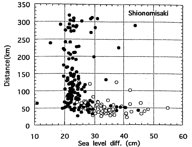
Fig. 3-5. Correlation between the position of the Kuroshio axis measured due southward from Cape Shionomisaki (in km) and the sea level difference between Kushimoto and Urakami (in cm). The distance was determined from the Prompt Report of Oceanographic Conditions published bimonthly by the Hydrographic and Oceanographic Department, Japan Coast Guard, and the sea level difference averaged for each half month is used. Black circles indicate the data which were taken at the time of a large meander and white circles those taken at the time of a straight path (Fujita 1997).
