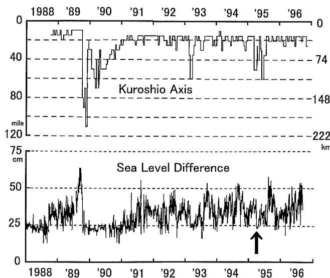
Fig. 3-23. Temporal variations of the position of the Kuroshio axis measured southward from Cape Shionomisaki (in nautical miles and in km), and the sea level difference between Kushimoto and Urugami (in cm: see Fig. 3-11 for the positions of these tide gauge stations). This sea level difference is usually used for monitoring the Kuroshio path off the Kii Peninsula (e.g., Kawabe, 1980).
