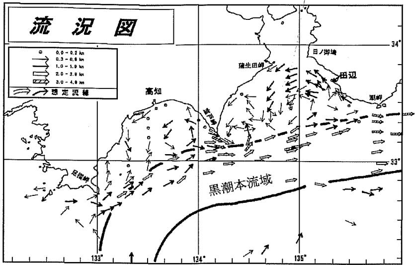
Fig. 5-7. Near surface current field based on ADCP observations conducted by various agencies in the area off Tosa Bay and the Kii Channel in the period from August 22 to 31, 1999. The observations include results of a special project conducted by the Fifth Maritime Safety Headquarter, and of routine observations conducted by the Marine Fisheries Experimental Station, Wakayama Research Center of Agriculture, Forestry and Fisheries. (Special Issue of Prompt Report of the Regional Oceanographic Condition published by the Maritime Safety Headquarters on September 1, 1999.) The scale of velocity vector is given in left top corner. Position of the current zone of the Kuroshio is shown with two bold curves.
