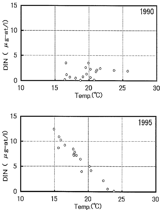
Fig. 5-24. Relation between water temperature ( ^{\circ}\text{C} ) and DIN ( \mu\text{g-at/l} ) observed in August 1990 (upper figure) and in August 1995 (lower figure).
