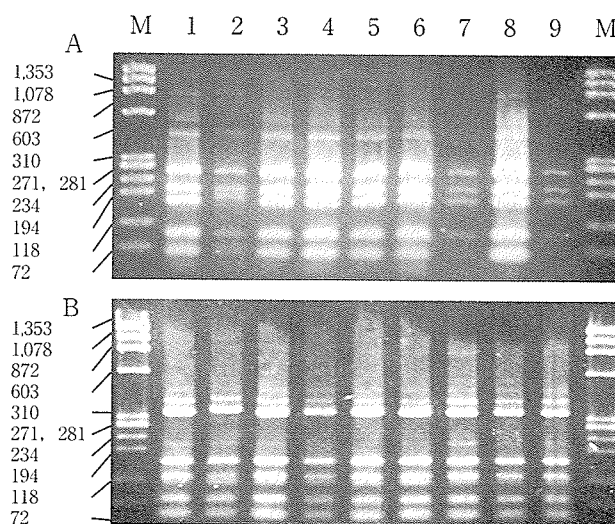
Fig. 3 Restriction fragment length profiles of the 16S-23S rDNA intergenic spacer regions amplified from A. ferrooxidans strains. Amplified products were digested with the restriction endonucleases, Hae III (A) and Alu I (B).
