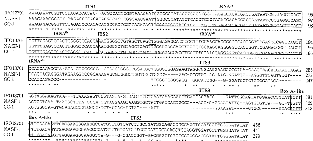
Fig. 2 Alignment of the 16S-23S rDNA intergenic spacer sequences from A. thiooxidans IFO 13701, A. ferrooxidans NASF-1, and A. caldus GO-1. Identical bases are indicated by asterisks and sequence gap are indicated by dashes.
