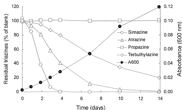
Fig. 3. Changes in the residual concentrations of s-triazines (simazine, atrazine, propazine, and terbuthylazine) in strain CDB21 culture supernatants. Residual concentrations of the s-triazines were expressed as the percentage of those in the blank culture. Growth of the cells was determined by measuring the absorbance at 600 nm. The details of the experiment conditions are described in Iwasaki et al. (2007).
