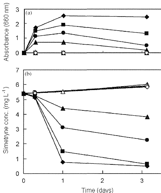
Fig. 5. Growth of strain JUN7 (a) and simetryn degradation by the isolate (b) in 1/10 (▲), 1/5 (●), 1/2 (■) and normal LB media (◆) supplemented with 5 mg L -1 of simetryn. White-colored symbols mean the respective uninoculated controls (modified from Harada et al. , 2006).
