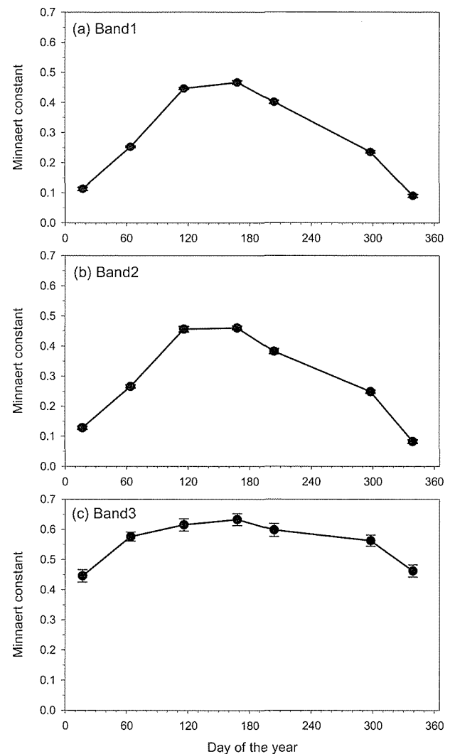
Fig. 5. The Minnaert constants derived from stratified random sampling, Sample II. Error bars represent standard deviations. (a) Band 1, (b) Band 2 and (c) Band 3.
