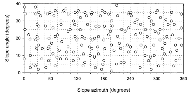
Fig. 4. Scattergram between slope azimuth and slope angle for the analysis of Sample II.
