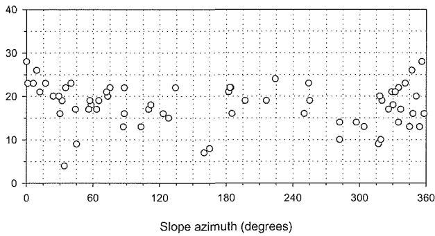
Fig. 2. Scattergram between slope azimuth and slope angle for the analysis of Sample I.
