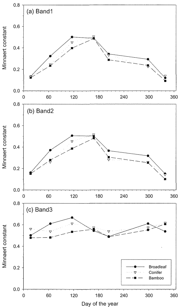
Fig. 3. The Minnaert constants for three forest types derived from same topographical features. (a) Band 1, (b) Band 2 and (c) Band 3.
