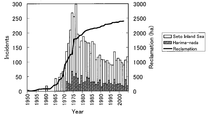
Figure 6. Long-term variations in incidents of red tides observed in Seto Inland Sea and Harima-Nada and area of reclaimed land in Harima-Nada.
