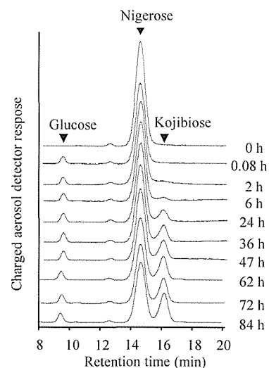
Fig 2. HPLC profiles during the conversion of nigerose into kojibiose.
