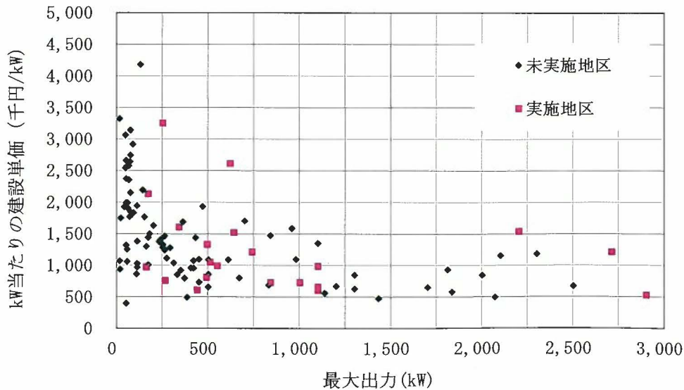
Fig.3 kW 当たりの建設単価と最大出力の関係 Relationship between the unit construction cost per kW and the maximum output
