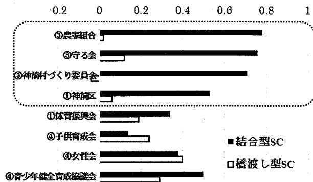
図3 各団体の保有する結合型SCと橋渡し型SC Fig.3 bonding SC and bridging SC which is holding by associations
