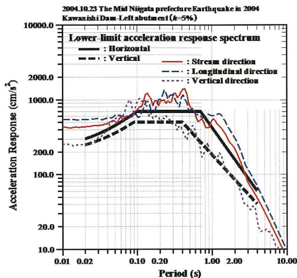
Fig. 18 加速度応答スペクトル (左岸地山) Acceleration response spectrum (Left abutment)
