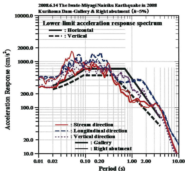
Fig. 32 加速度応答スペクトル (基部監査廊と下流右岸地山) Acceleration response spectrum (Gallery and right abutment)
