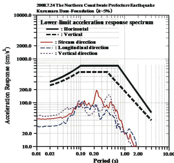
Fig. 40 加速度応答スペクトル(河床部監査廊) Acceleration response spectrum (Foundation)
