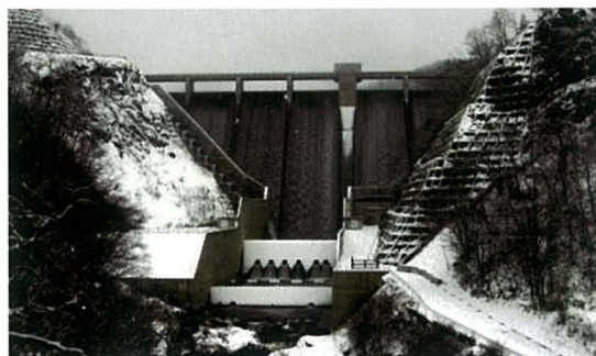
Fig. 41 大志田ダム Overall view of Ooshida Dam
