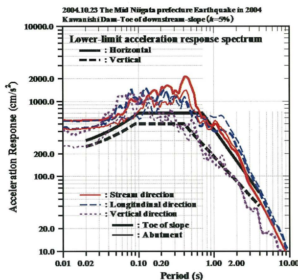
Fig. 19 加速度応答スペクトル (下流法尻と左岸地山) Acceleration response spectrum (Toe of downstream-slope and left abutment)
