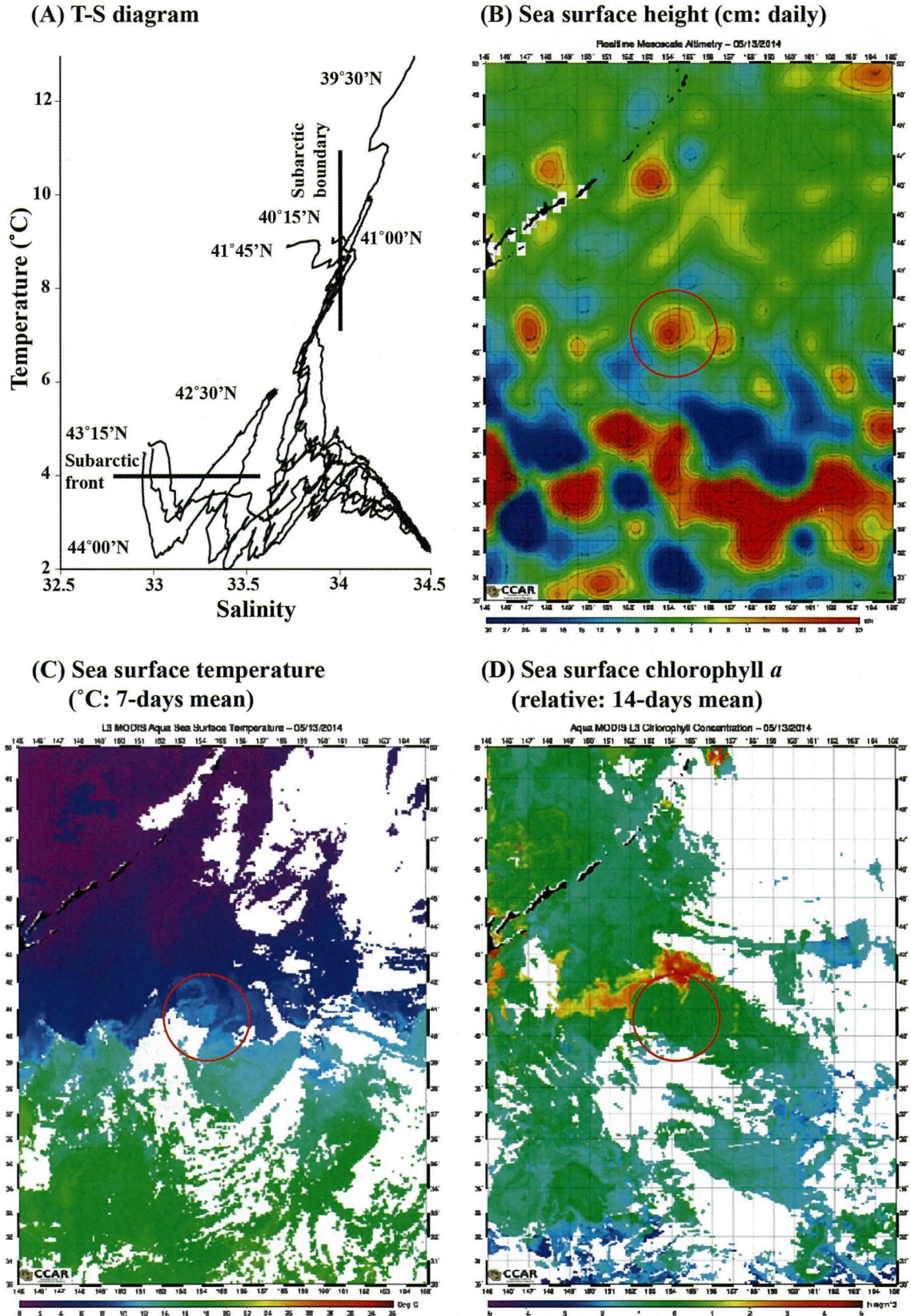
Fig. 6. T-S diagram of data obtained at seven stations along the 155°E line (A), the sea surface height (B), sea surface temperature (C) and chlorophyll a levels (D) in the western North Pacific from May 8 to 19, 2014. The data for (B)–(D) were obtained from Colorado University ( http://eddy.colorado.edu/ccar/ssh/nrt_global_grid_viewer ). The positions of the subarctic front (i.e., the 4°C isotherm line) and subarctic boundary (the 34 isohaline line) are shown in (A). The circles in (B)–(D) indicate the approximate positions of the warm core detected by satellite data.
