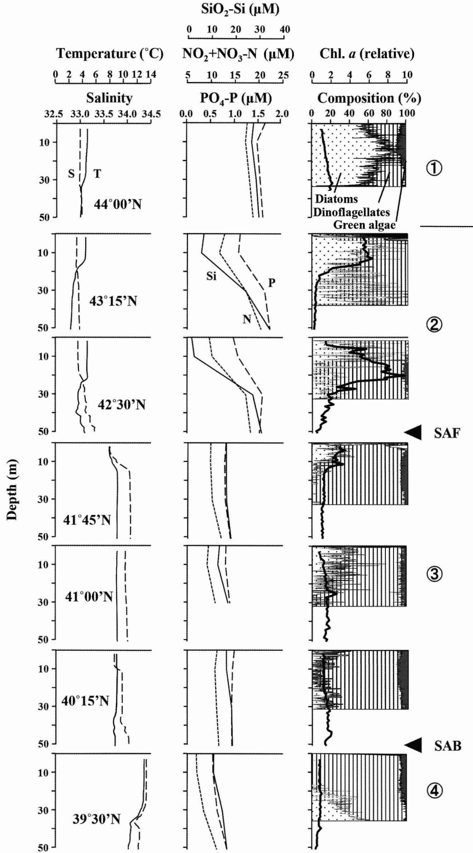
Fig. 4. The vertical distribution of temperature and salinity (left), inorganic nutrients (middle) and chlorophyll a and their taxonomic compositions (right) at seven stations along the 155°E line in the western North Pacific from May 8 to 19, 2014. The solid arrow heads indicate the positions of the Subarctic Front (SAF) and Subarctic Boundary (SAB) (cf. Fig 3). The circled numbers in the right column indicate the four types of phytoplankton communities along the 155°E line.
