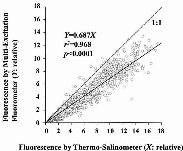
Fig. 2. Comparison between multi-excitation fluorometer-derived fluorescence ( Y ) and thermo-salinometer-derived fluorescence ( X ) for the total pigments identified via in situ multi-excitation fluorometer in the western North Pacific along the track of the T/S Oshoro-Maru cruise from May 8 to 19, 2014. The dashed line indicates positions along the line Y=X (1 : 1).
