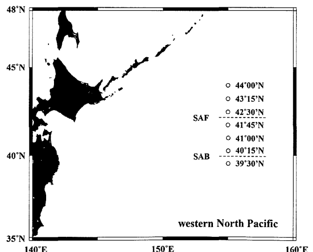
Fig. 1. The location of the sampling stations along the 155°E line in the western North Pacific from May 8 to 19, 2014. Approximate positions of the Subarctic Front (SAF) and Subarctic Boundary (SAB) are shown using broken lines (cf. Fig. 3).
