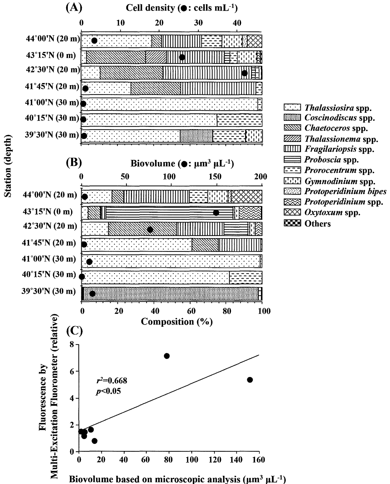
Fig. 5. Results of a microscopic analysis. Species composition in terms of phytoplankton cell density (A) and biovolume (B) at the fluorescence peak depth of each station along the 155°E line in the western North Pacific from May 8 to 19, 2014, are indicated. The relationship between fluorescence evaluated by in situ multi-excitation fluorometry and the biovolume quantified by microscopic analysis is shown (C).
