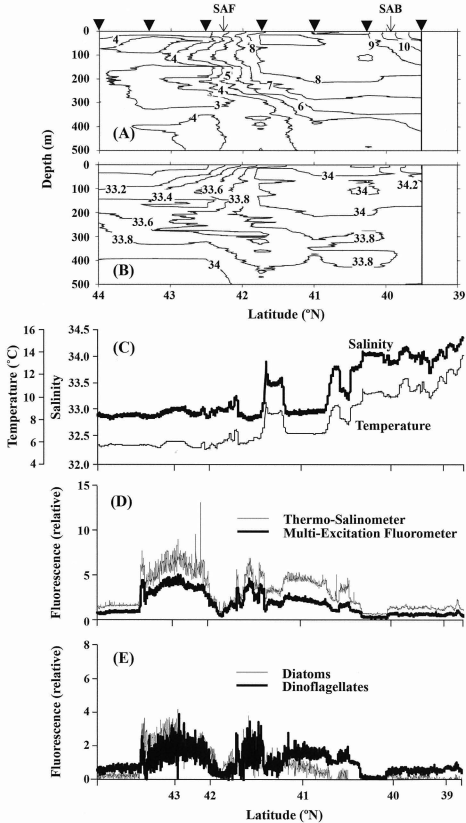
Fig. 3. Latitudinal changes in the vertical dimension of temperature (A) and salinity (B), surface temperature and salinity (C), total fluorescence detected by in situ multi-excitation fluorometer and thermo-salinometer (D), and diatom and dinoflagellate fluorescence detected by in situ multi-excitation fluorometer (E) in the western North Pacific along 155°E from May 8 to 19, 2014. The solid triangles in (A) indicate sampling stations. The positions of the Subarctic front (SAF) and Subarctic boundary (SAB) are shown with arrows in (A).
