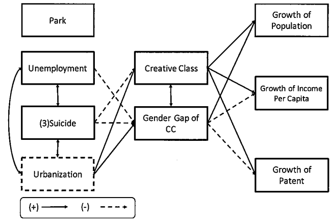
Fig. 5. Path Diagram (3): Suicide
