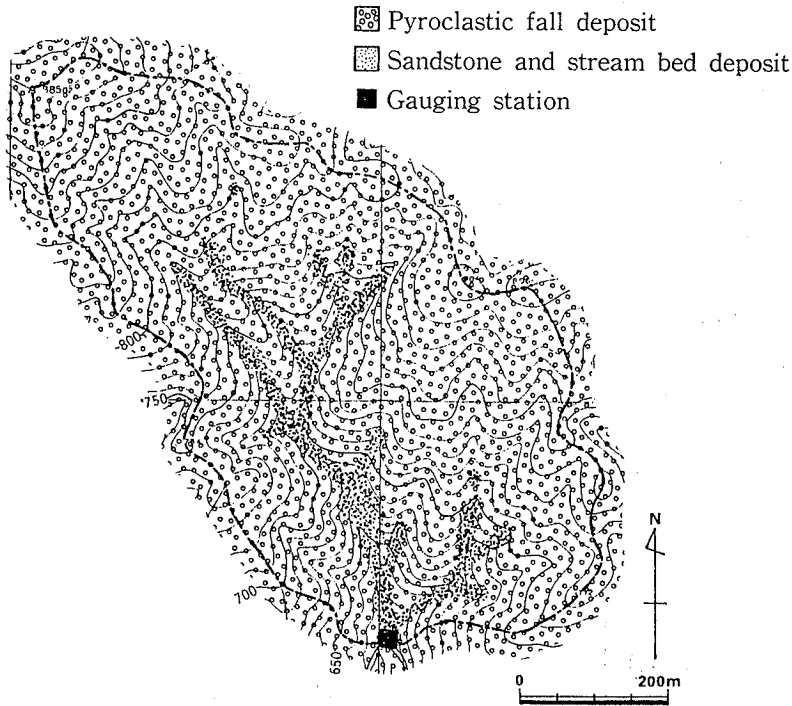
Fig. 2 Topography and geology of No. 2 Takakuma basin.
