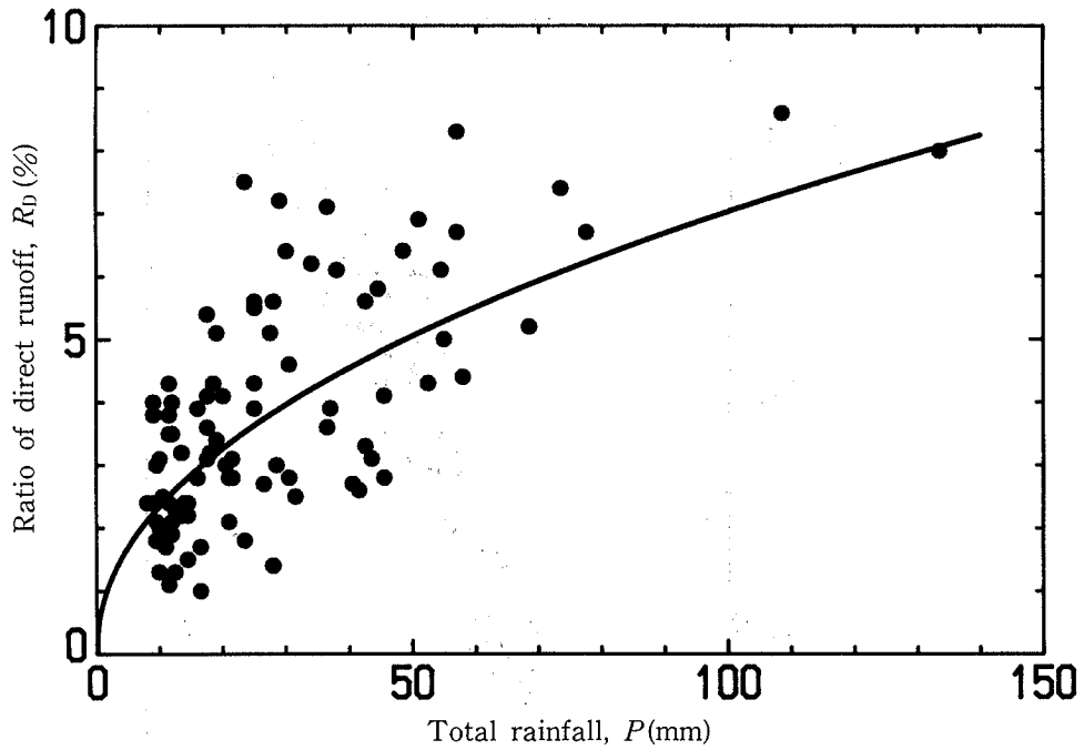
Fig. 11 Relationship between total rainfall and ratio of direct runoff.
