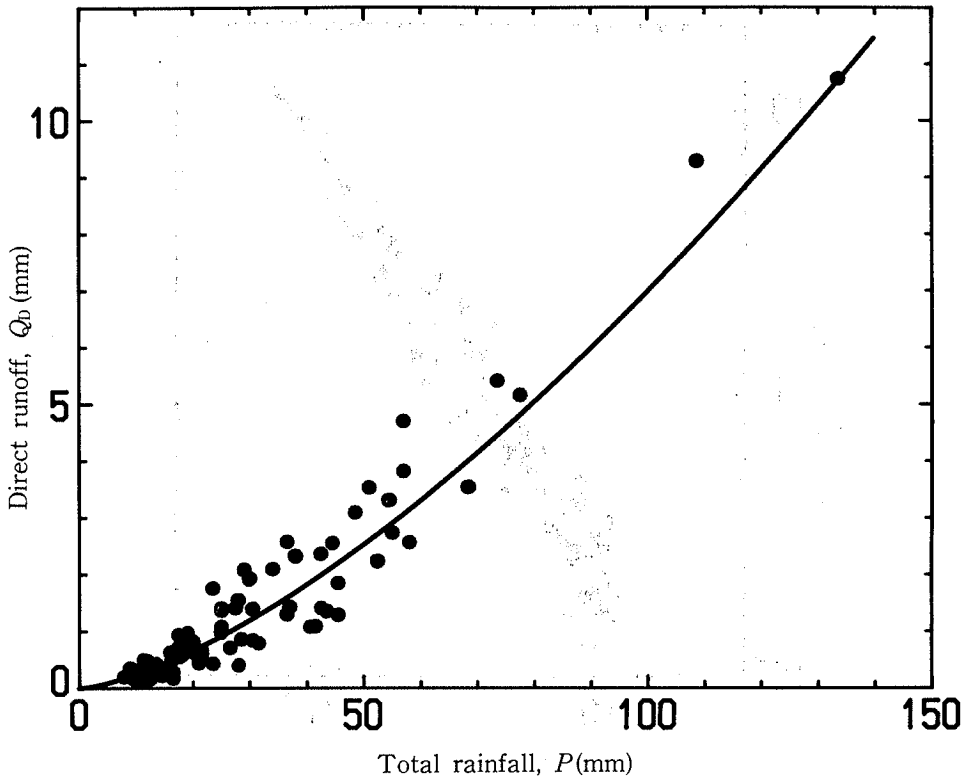
Fig. 9 Relationship between total rainfall and direct runoff.
