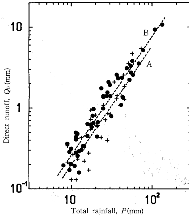
Fig. 10 Relationship between total rainfall and direct runoff (at logarithmic paper).
