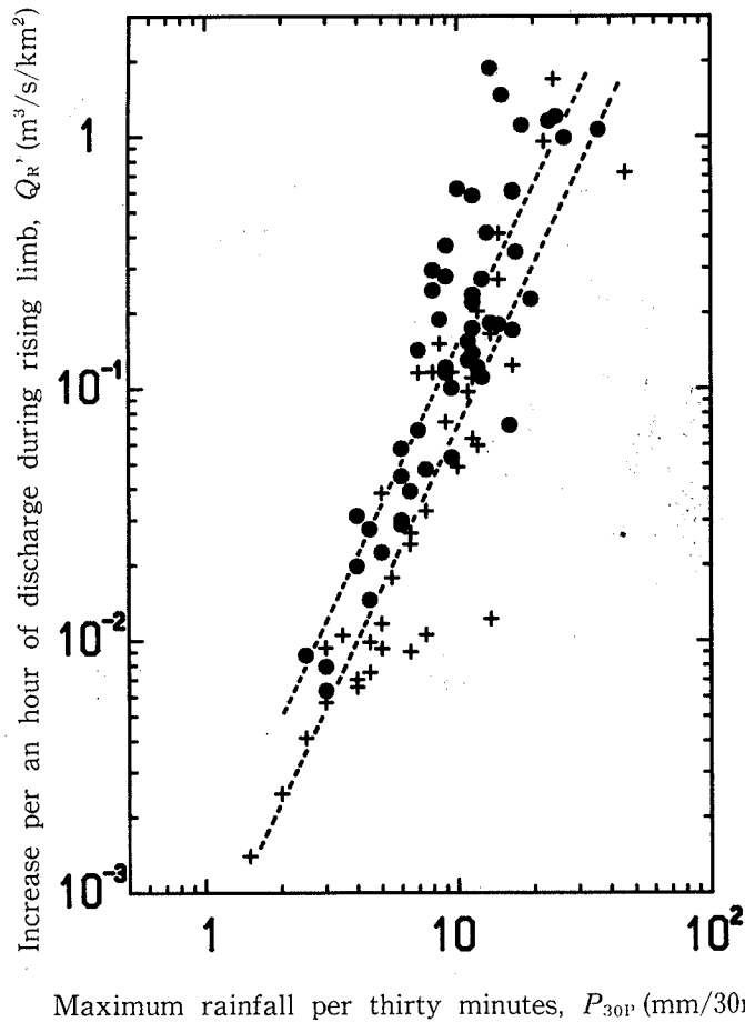
Fig. 13 Relationship between rainfall intensity and increase per an hour of discharge during rising limb.
