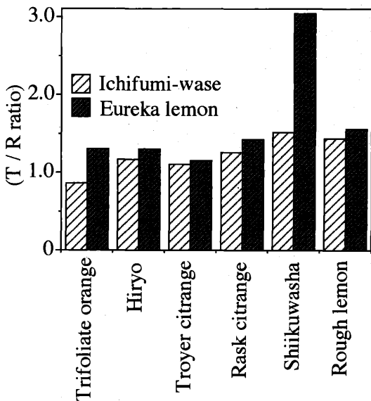
Fig. 4. Top-Root ratios of six rootstocks grafted with 'Ichifumi-wase' and 'Eureka' lemon scions, 20 months after grafting.
