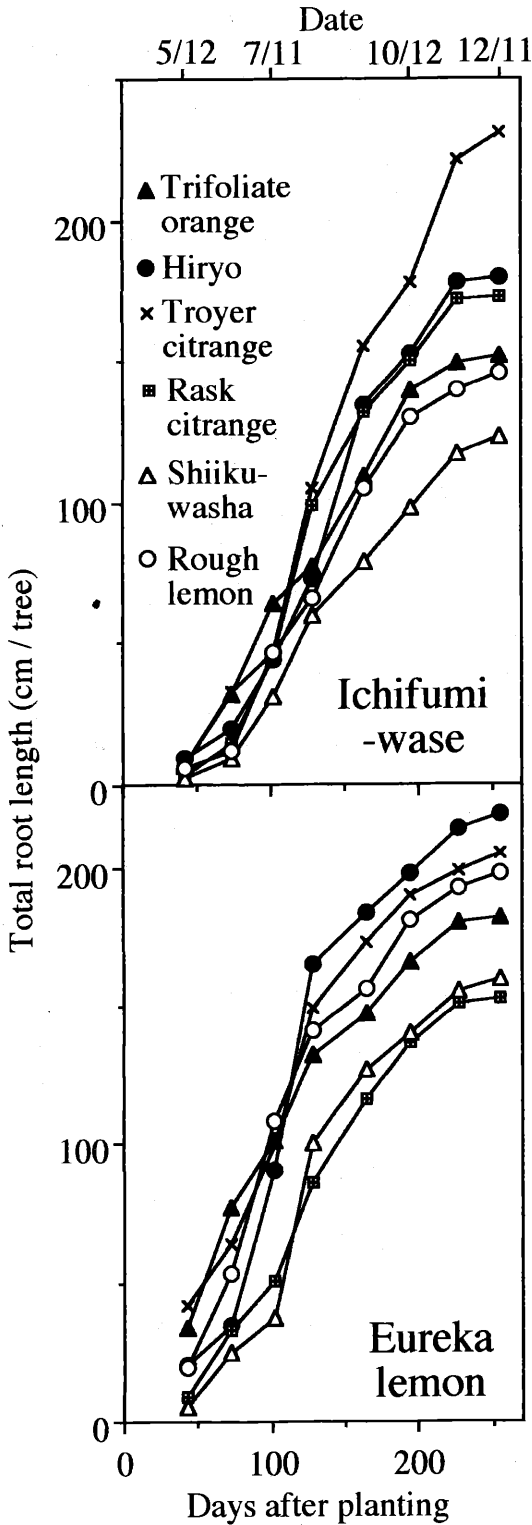
Fig. 2. Growth curves of rootstocks grafted to tow different scion tops, 42 to 255 days after planting.
