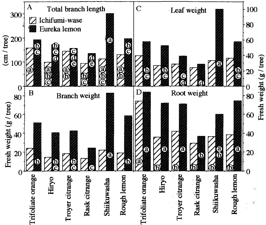
Fig. 3. Total branch length (A), branch weight (B), leaf weight (C) and root weight (D) of six rootstocks grafted with 'Ichifumi-wase' and 'Eureka' lemon scions, 20 months after grafting. 2 Mean separation by Duncan's multiple range test, 1% level, except for total branch length in 'Ichifumi-wase' (A), 5% level.
