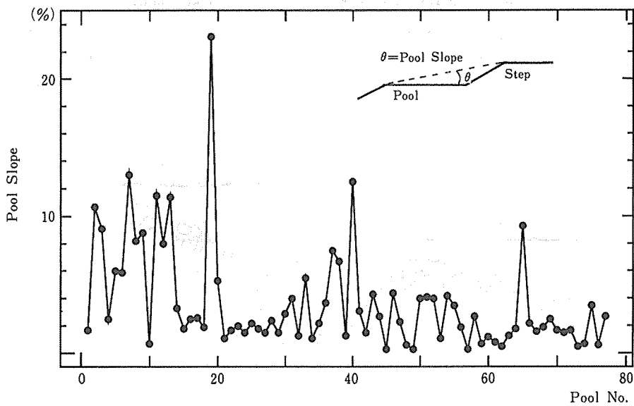
Fig. 4 Change of pool slope ( \theta ) in the research channel.
