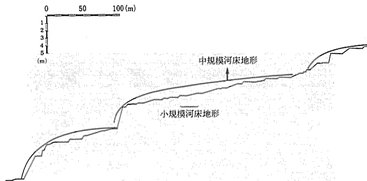
Fig. 5 Classification of channel morphology of a series of pool-step bed forms.
