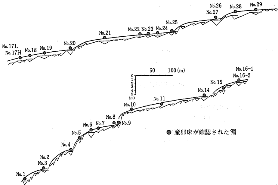
Fig. 3 Profile of morphology in the channel for fish observation.
