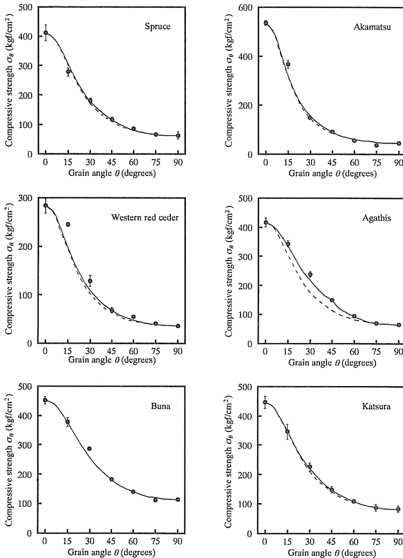
Fig. 1. Compressive strengths corresponding to the grain angles. Legend: Solid dots: Mean, Horizontal bars: Standard deviation, Solid lines: Modification of Hankinson's formula, Dashed lines: Conventional Hankinson's formula. Notes: Both predictions for Buna are almost overlapped.
