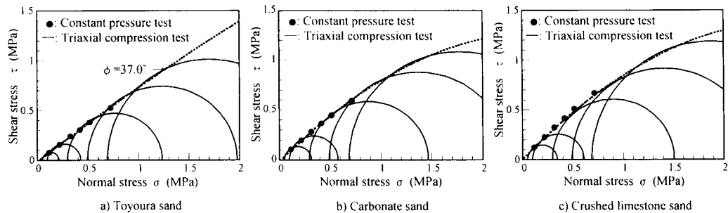
Fig.9 Comparison of failure envelope for direct shear test and triaxial compression test
