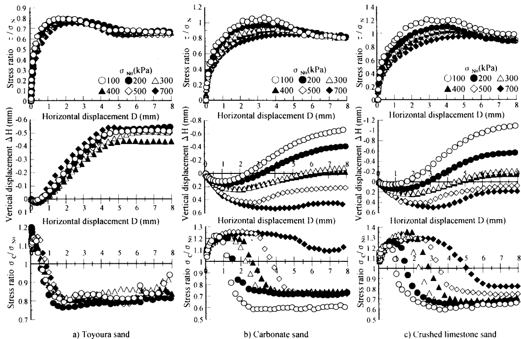
Fig. 3 Result of constant pressure test by using improved apparatus
