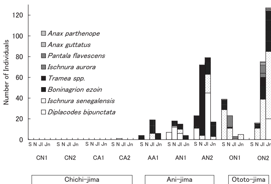
Fig. 3. Number of odonate individuals collected in nine sampling stations of three islands. S: September, N: November, JI: July, Jn: June.
