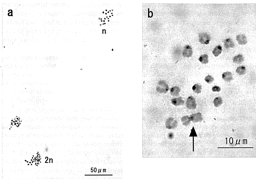
Fig. 5. Chromosomal mosaicism found in a blastocyst derived from an in vitro -fertilized mouse oocyte. Three metaphases, two diploid blastomeres (at the lower left), and one haploid blastomere (at the upper right) can be observed in this photo (a). High magnification of the haploid metaphase (b). An arrow shows the translocation chromosome, indicating that this haploid blastomere originated from an odd fertilized sperm.
