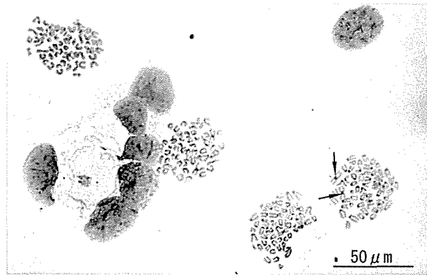
Fig. 4. Sample chromosome from a triploid blastocyst at 96 h after insemination. This embryo was derived from a prepubertal mouse oocyte fertilized in vitro . There are two translocated chromosomes in each metaphase (arrows). Therefore, this embryo originates from polyspermy.
