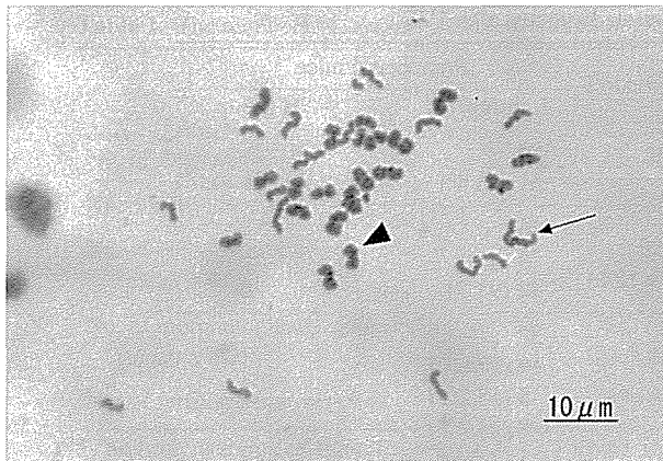
Fig. 3. Premature chromosome condensation (PCC) from a sperm and female chromosomes at the M-II stage in a 1-cell arrested embryo derived from a prepubertal mouse at 31 h after IVF. An arrow shows PCC of the translocation chromosome from a RF male mouse. Male chromosomes showing single chromatids as PCC are different from female chromosomes showing bivalent chromosomes at the M-II stage indicated by an arrowhead.
