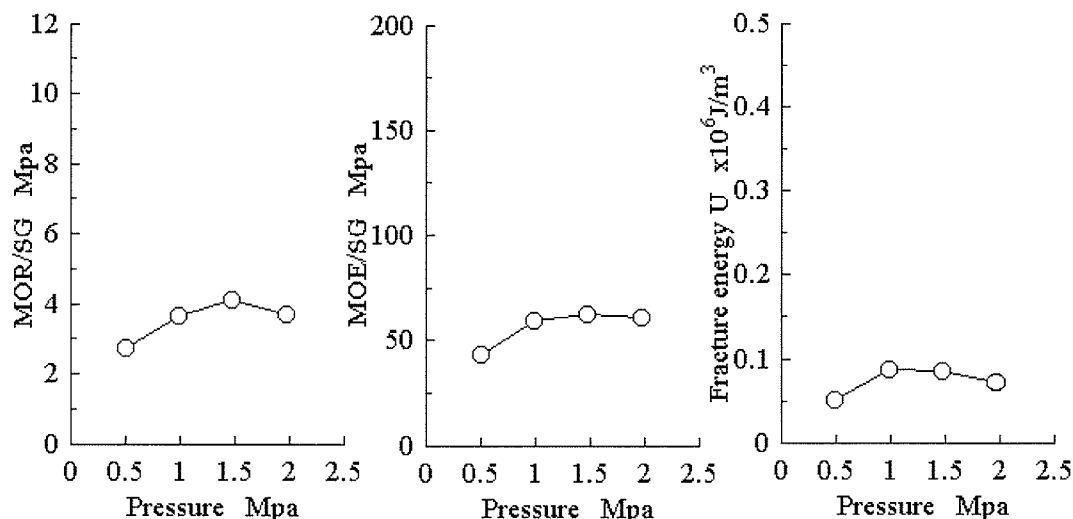
Fig. 2 Relationship between hot-press pressure and bending characteristics of epoxy-bonded boards. Note: Wood:Filler:Resin=50:20:30 Press time:30 min
