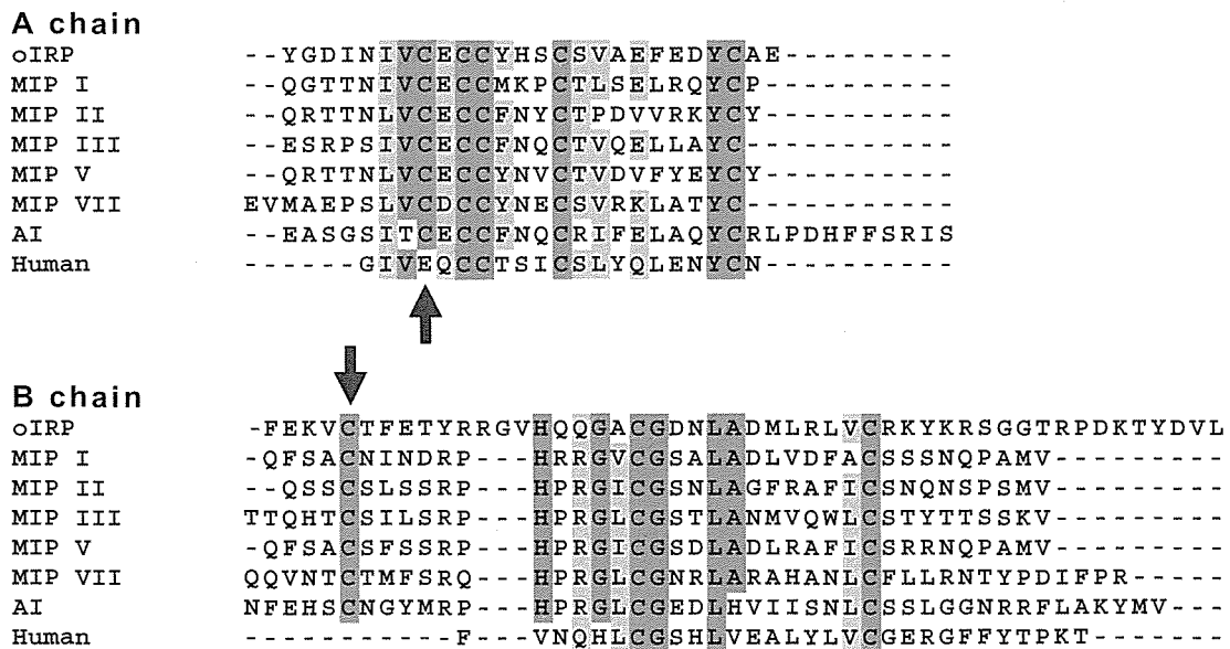
Fig. 1. Amino acid sequence comparison of the insulin-related peptides of mollusks with human insulin. The positions that have an identical residue or similar amino acids are shaded with dark or light grey respectively. Arrows indicate the extra cystein residues of the molluscan insulin. oIRP, Pacific oyster insulin-related peptide; MIP, molluscan insulin-related peptide of Lymnaea stagnalis ; AI, Aplysia insulin; Human, human insulin.
