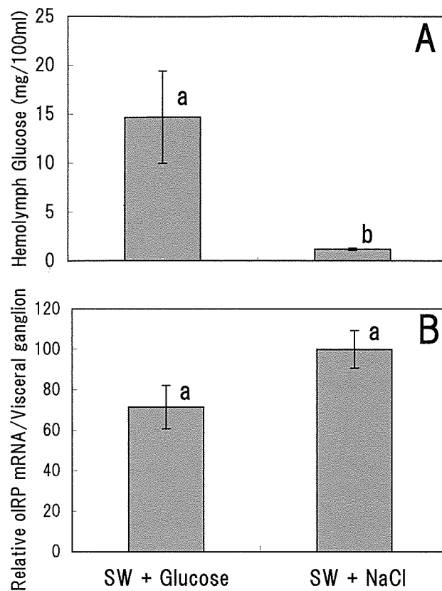
Fig. 3. Effects of glucose administration on the hemolymph glucose concentration (A) and the oIRP mRNA level in the visceral ganglion (B) of the Pacific oyster. Oysters were immersed in the seawater containing 20 mM glucose or 10 mM NaCl for 90 min at 14 °C. Each column with a vertical bar represents the mean \pm SEM. Groups sharing a common letter do not differ significantly ( p > 0.05 ).
