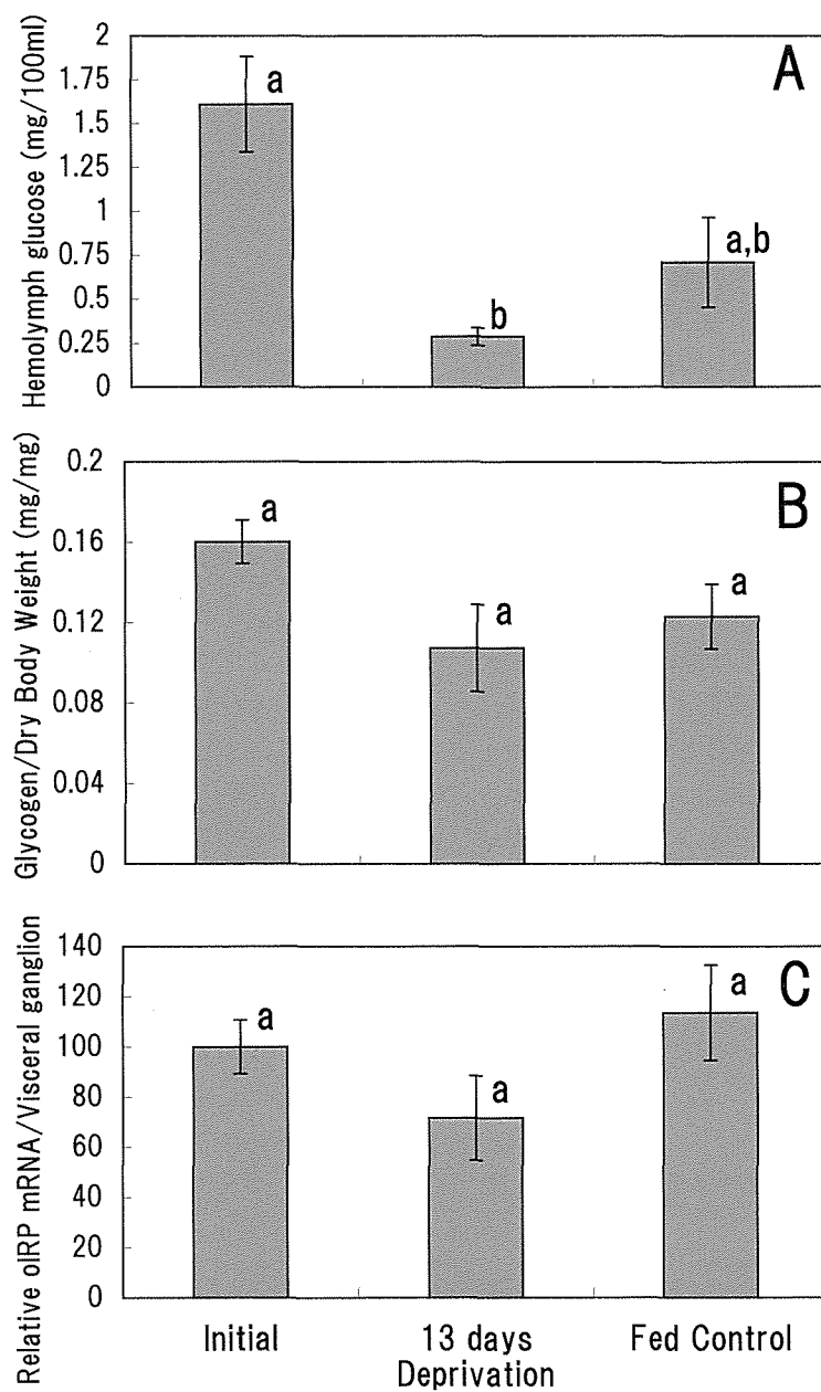
Fig. 2. Effects of food deprivation on the hemolymph glucose concentration (A), glycogen content of the dry meat (B), and the oIRP mRNA level in the visceral ganglion (C) of the Pacific oyster. Each column with a vertical bar represents the mean \pm SEM. Groups sharing a common letter do not differ significantly ( p > 0.05 ).
