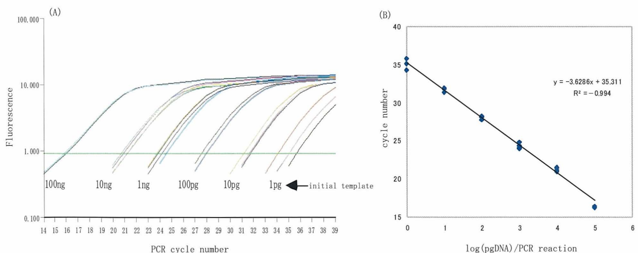
Fig. 2. (A) Amplification curve of real-time PCR. Y axis is SYBR Green I fluorescence. X axis is PCR cycle number. Arrow indicates initial template concentrations of P. pulmonarius DNA. (B) Correlation between the log of DNA concentration and threshold cycle number ( n = 3 ). Y axis is cycle number. X axis is log of DNA concentration.
