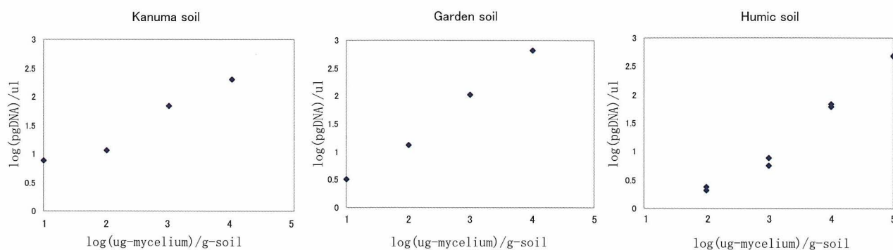
Fig. 4. Correlation between log of DNA concentration and log of mycelial mass (Kanuma soil, garden soil: n = 1 ; humic soil: n = 2 ).
