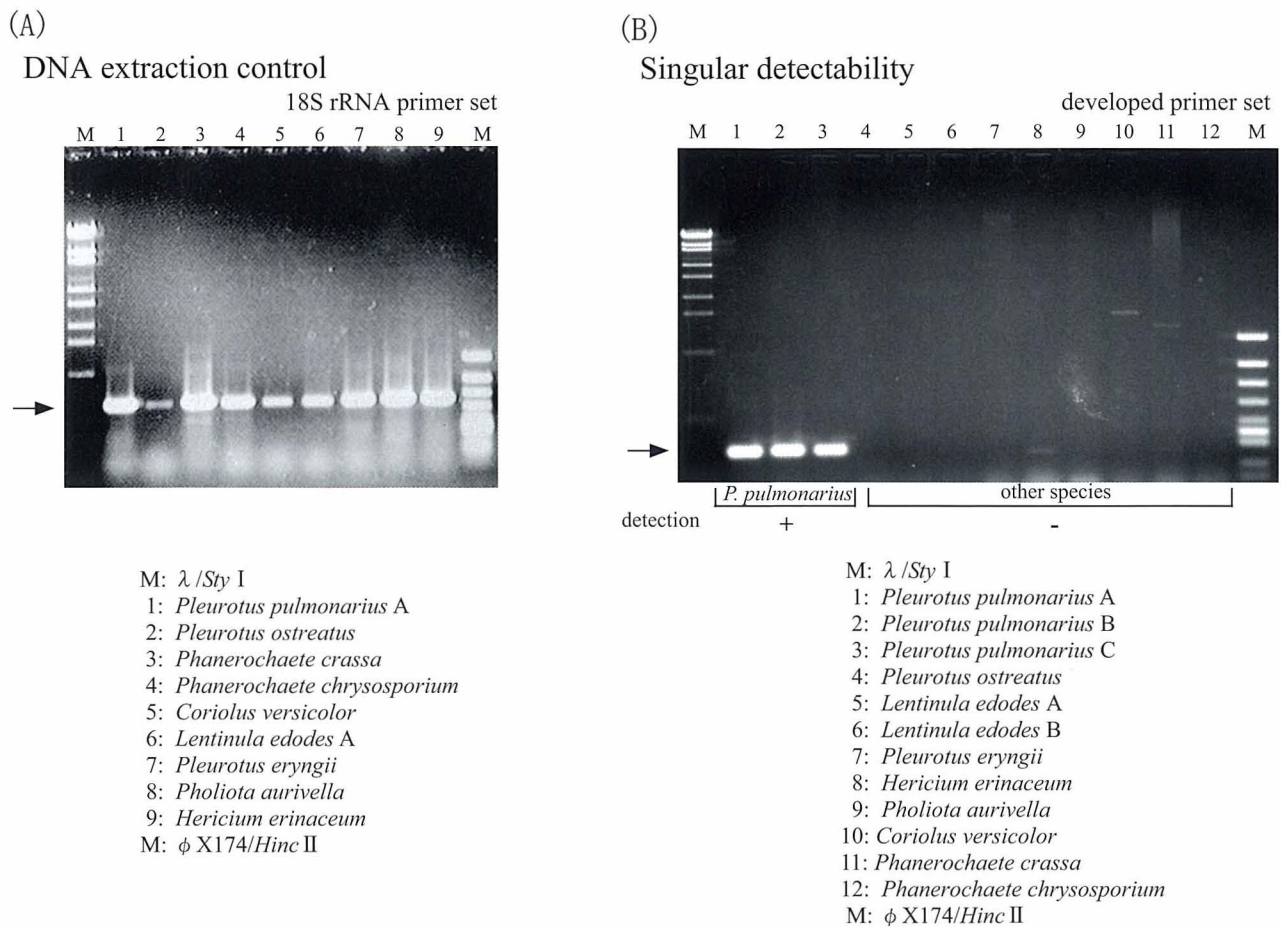
Fig. 1. (A) DNA extraction control. DNA was extracted by the CTAB method from Pleurotus pulmonarius and other eight white-rot fungi. (B) Amplification of extracted DNAs by PCR with the primer set designed for Pleurotus pulmonarius .
