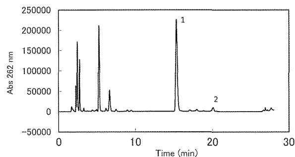
Fig. 2 Chromatogram of the latex collected from crisp-head lettuce, 'Falcon'.
