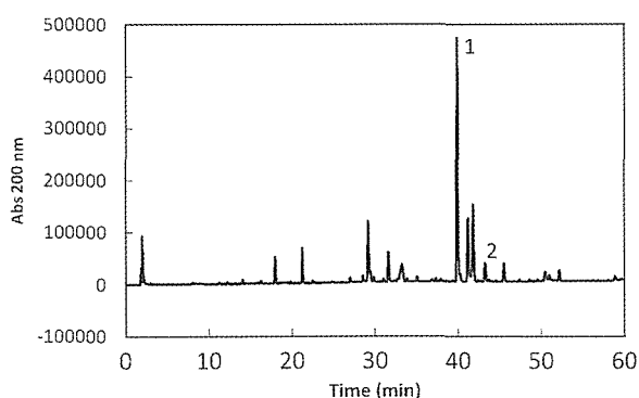
Fig. 1 Chromatogram of the latex collected from crisp-head lettuce, 'Falcon'.
