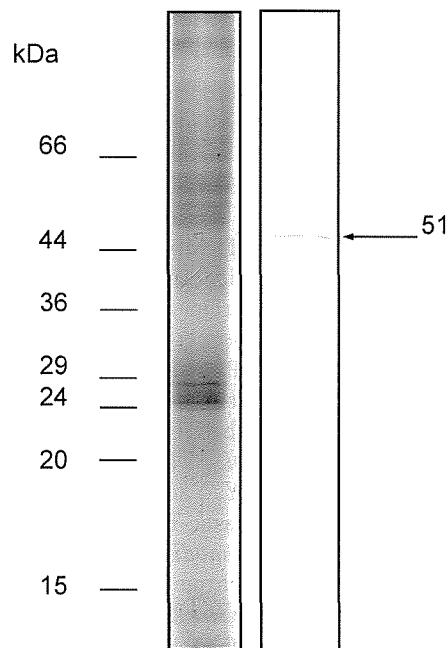
Fig. 6 Immunochemical detection of 51 kDa protein band in SDS-gel with anti-GNTI-PL antisera. The isolated NDPase-associated Golgi membranes were subjected to SDS-PAGE, followed by immunoblotting with anti-GNTI-PL antisera. Details of experiments are described in the text.
