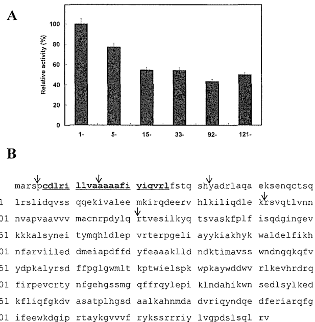
Fig. 5 Activity expression of N -terminal truncated GNTI-PL. (A) Activities of the truncated enzymes. (B) Diagram of the truncated GNTI-PL. Underlined bold type, transmembrane domain; arrows, the truncated sites.
