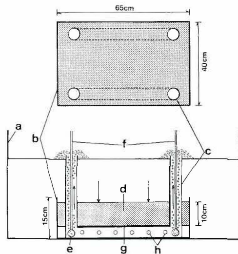
Fig. 23. Schematic drawing of the estivation bed used in the rearing experiment. a: 2 ton-tank, b: plastic container, c: vinyl chloride pipe ( \phi = 25 mm), d: sand (particle size = 1-2 mm), e: air stone, f: air tube, g: net (mesh size = 0.5 mm), h: water absorptive ports.
