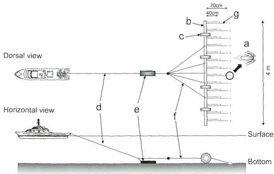
Fig. 25. Schematic drawing of the karatsurikogi fishing gear used for collecting Japanese sand lance under estivation in the mouse of Ise Bay. a: hook, b: stainless steel bar ( \phi 22 mm), c: float, d: rope ( \phi 20 mm), e: iron weight (10 kg), f: rope ( \phi 12 mm), g: rope ( \phi 4 mm).
