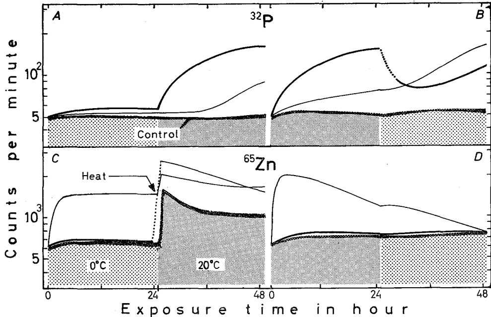
Fig. 4. The uptake curves of ^{32}\text{P} and ^{65}\text{Zn} as the functions of time and temperature. Broad line: living, narrow line: heat killed, ▨: control 1, ▤: 0°, ▩: 20°C. A: Micrococcus , B: T. dattila , C: R. mucilaginosus , D: Pseudomonas I .
